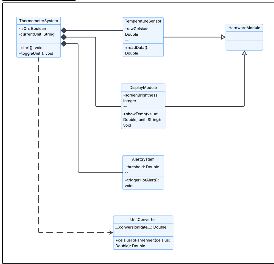
Digital Thermometer System - UML Class Diagram
