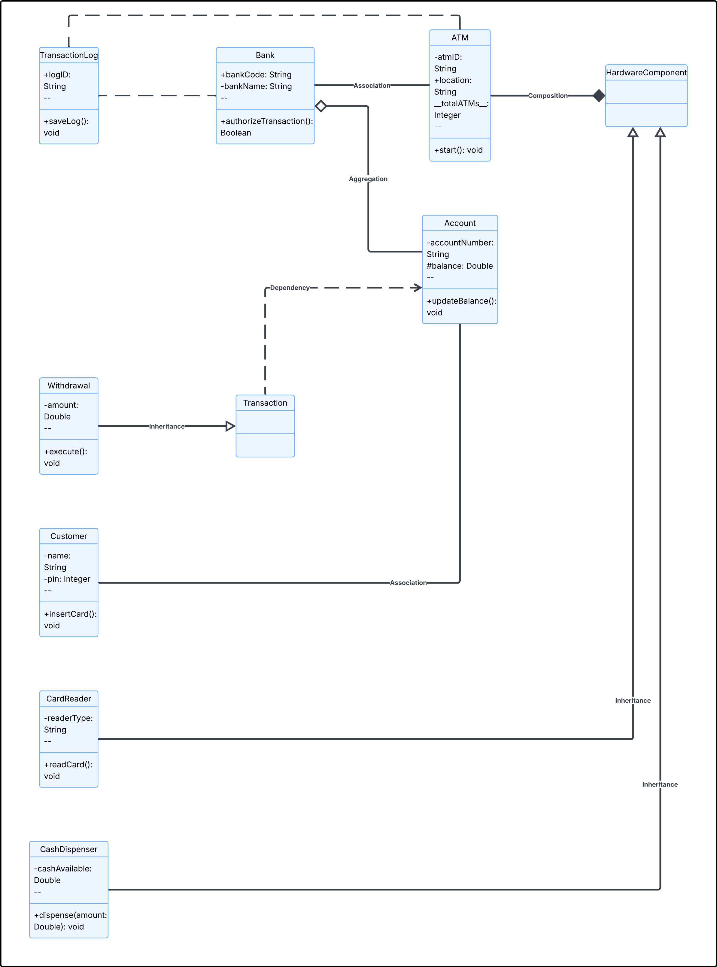
ATM System: Strict UML Class Diagram
