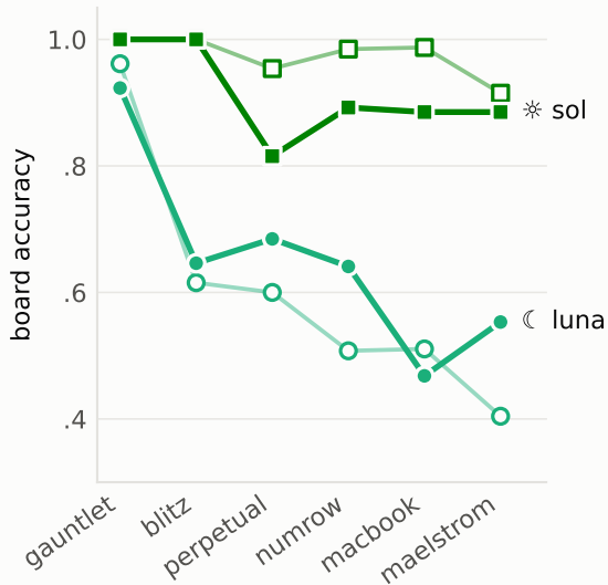
(a) Accuracy
