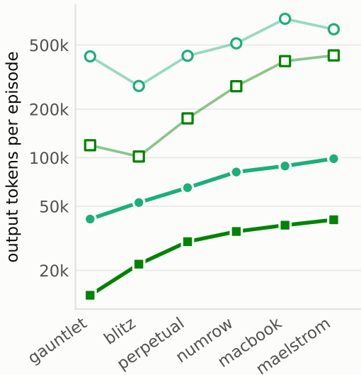
(b) Output tokens, log scale
