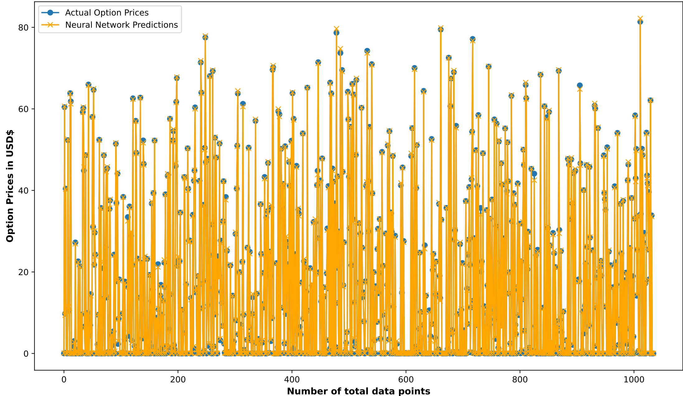
Project 1. Actual Call Option Price vs Neural Network Predictions, "Baseline" ANN - 3L 150N, SGD optimizer, 1035 point training set with momentum
