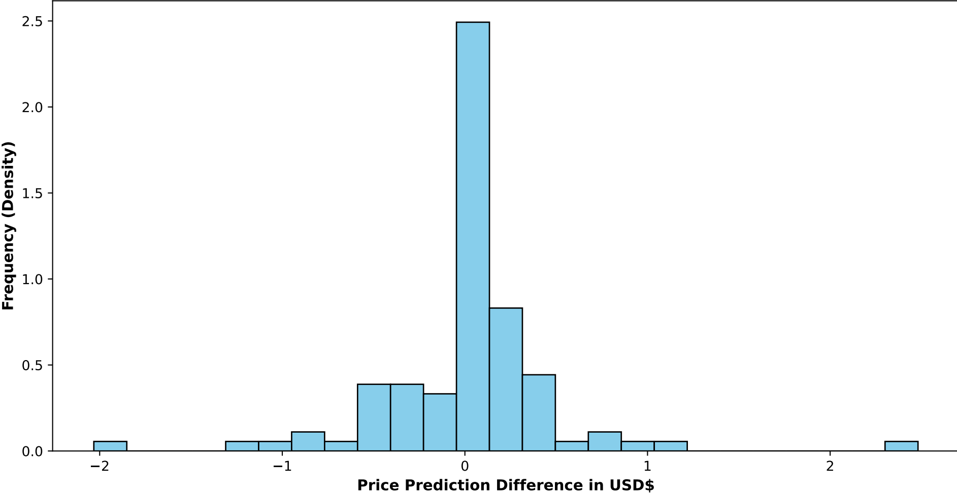
Project 1. Histogram of Prediction Differences Expanded ANN - 7L 150N, Adam optimizer, 1035 data point training set, 100 data point test set
