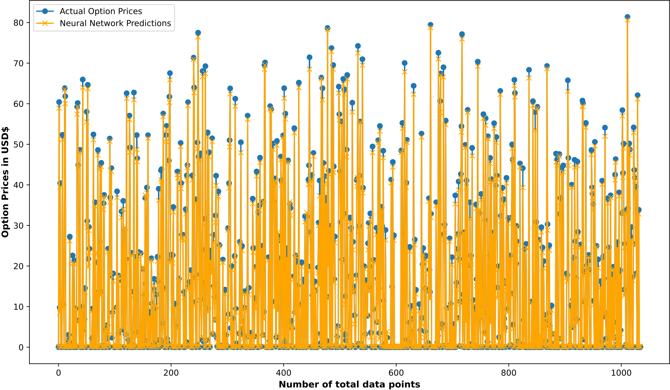
Project 1. Actual Call Option Price vs Neural Network Predictions, "Baseline" ANN - 3L 150N, SGD optimizer, 1035 point training set without momentum
