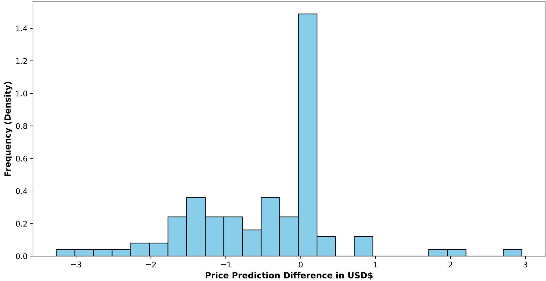
Project 1. Histogram of Prediction Differences Baseline ANN -3L 150N, SGD optimizer, 1035 point training set, 100 point test set without momentum
