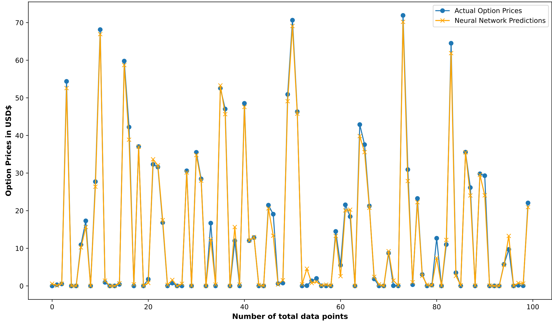
Project 1. Actual Call Option Price vs Neural Network Predictions, "Expanded" ANN - 7 Layers 700 Neurons, SGD optimizer, 1035 data point training set, test 100 data points
