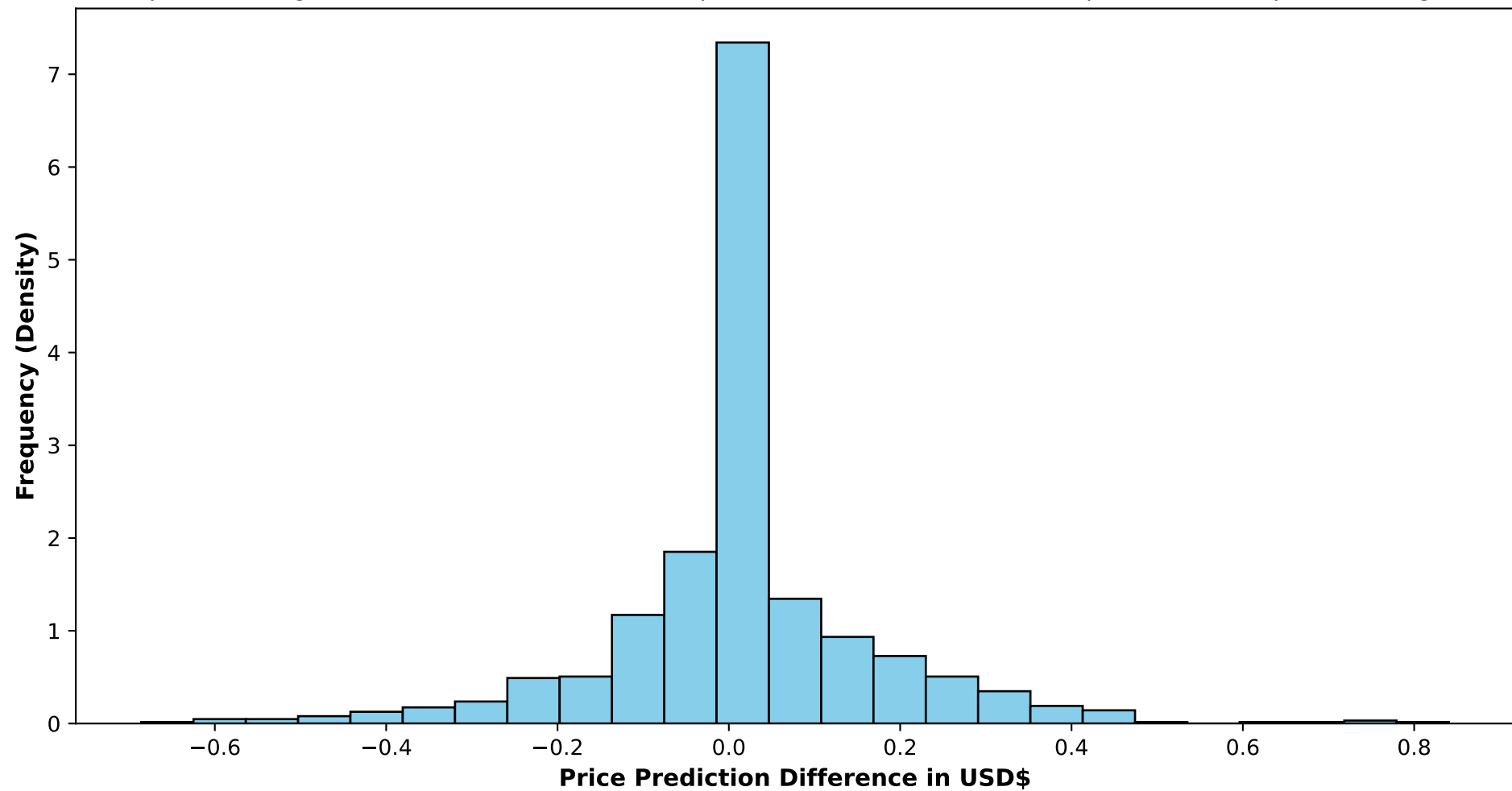
Project 1. Histogram of Prediction Differences "Expanded" ANN - 7L 700N, Adam optimizer, 1035 point training set
