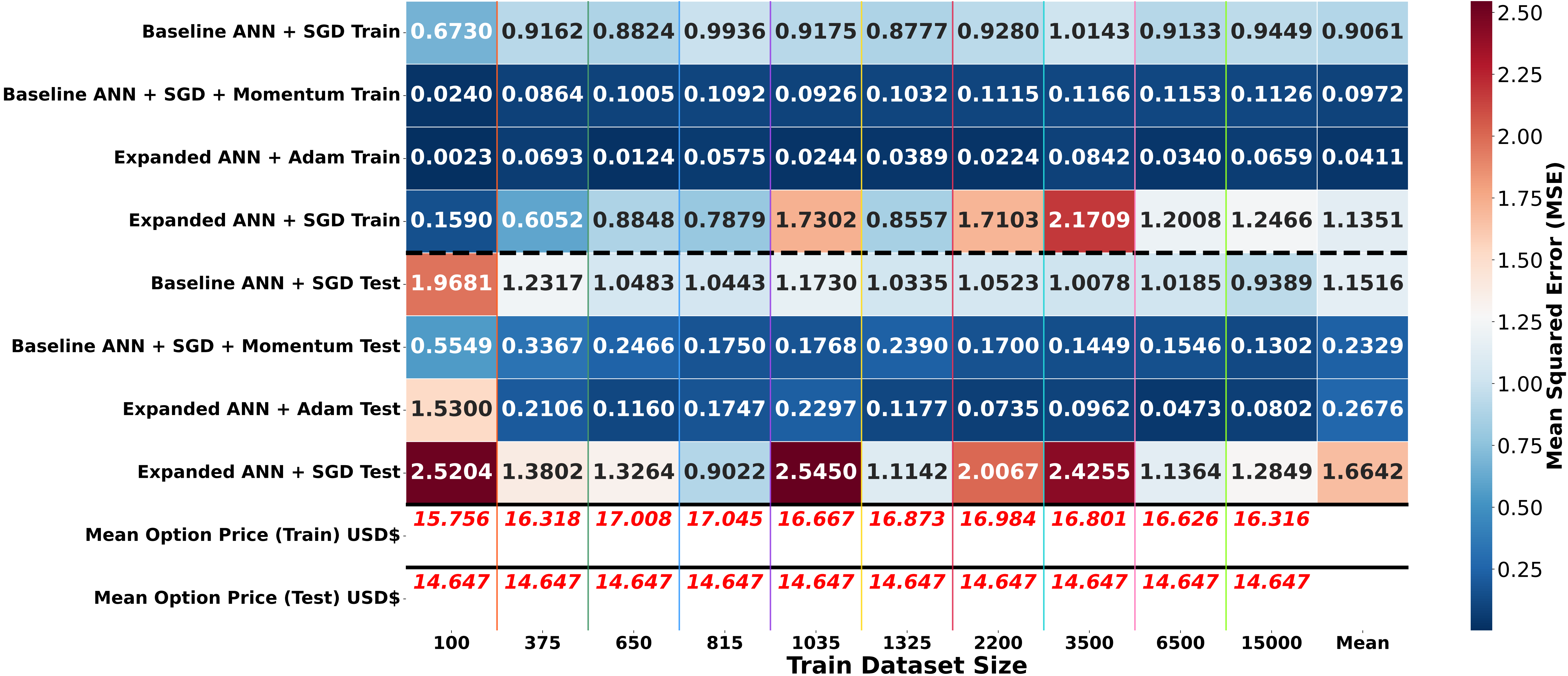
Project 1: Mean Squared Error (MSE) — Train vs Independent Test (100 data points) Baseline ANN (3 layers, 150 neurons) vs Expanded ANN (7 layers, 700 neurons) (Momentum = 0.8)
