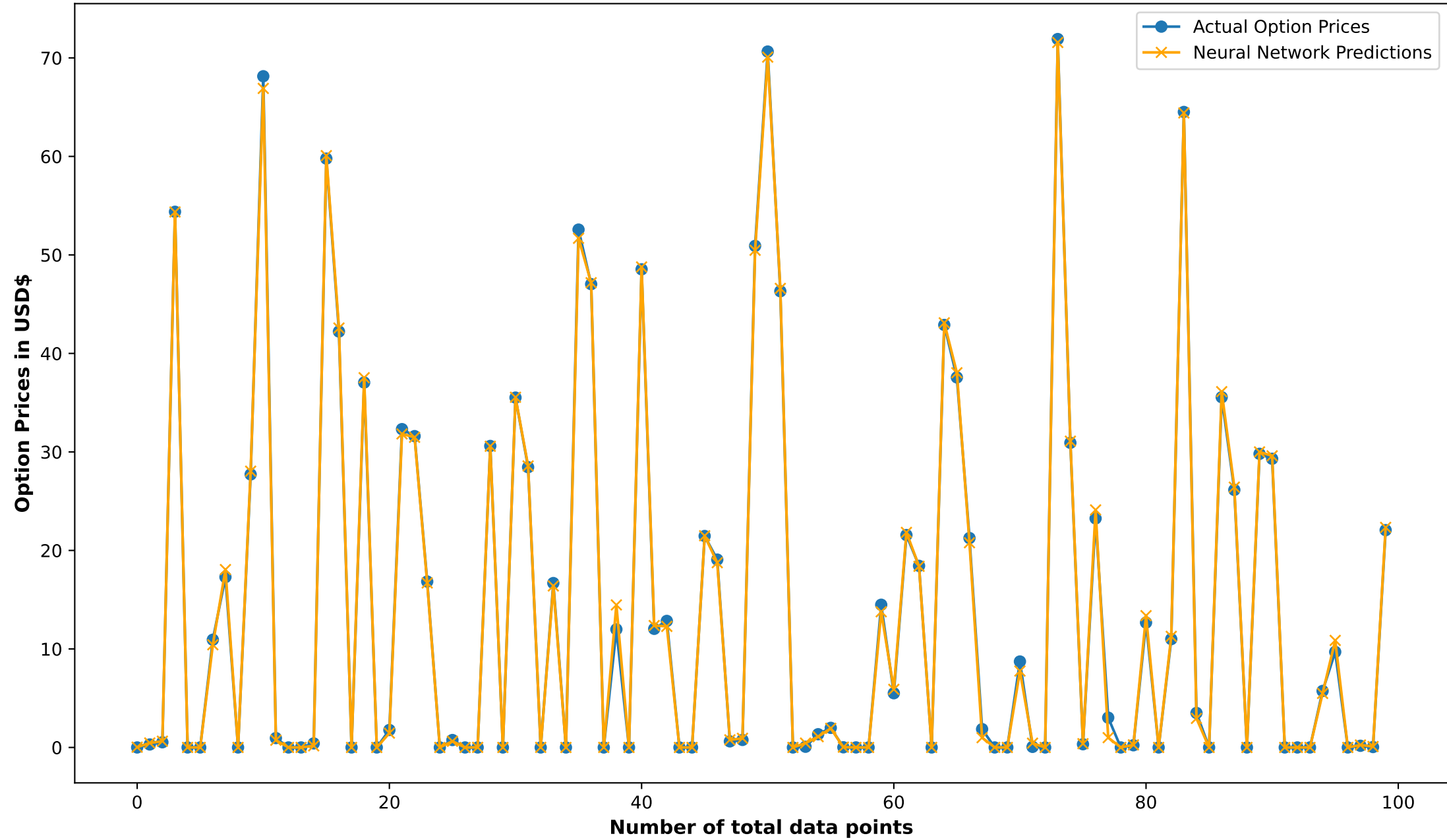
Project 1. Actual Call Option Price vs Neural Network Predictions, Expanded ANN - 7L 150N, Adam optimizer, 1035 data point training set, 100 data point test set
