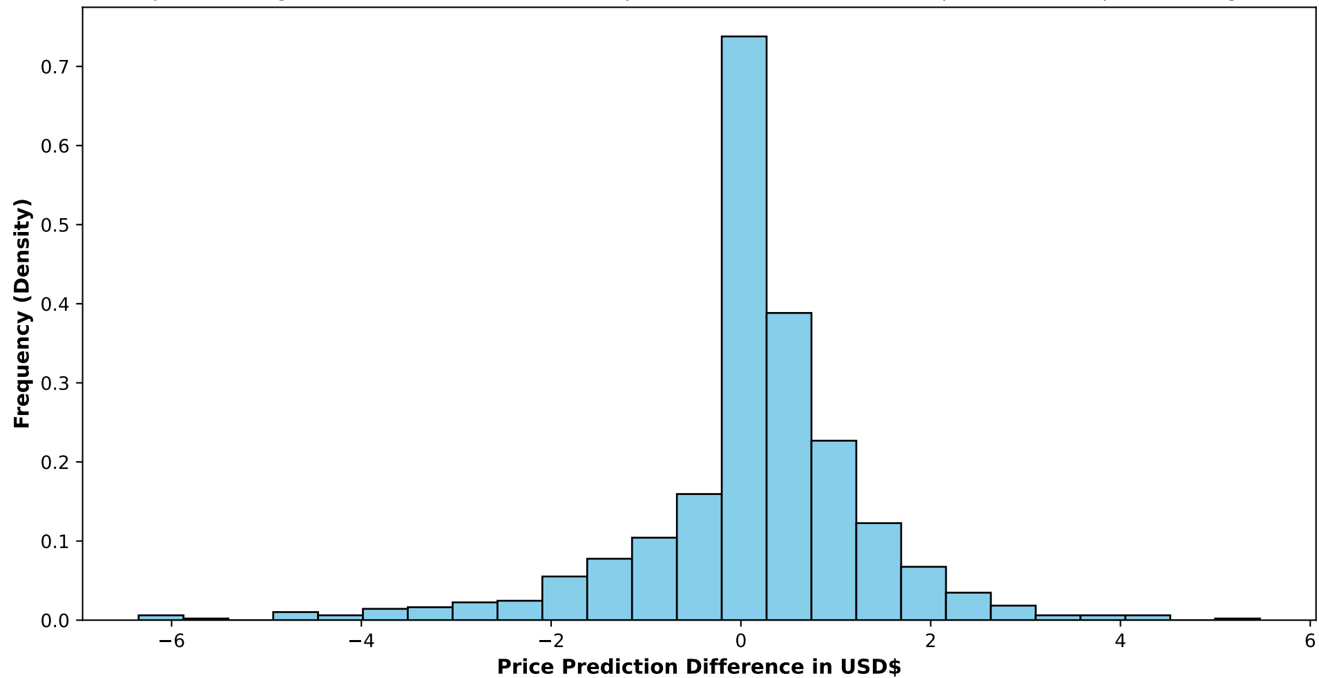
Project 1. Histogram of Prediction Differences "Expanded" ANN - 7L 700N, SGD optimizer, 1035 point training set
