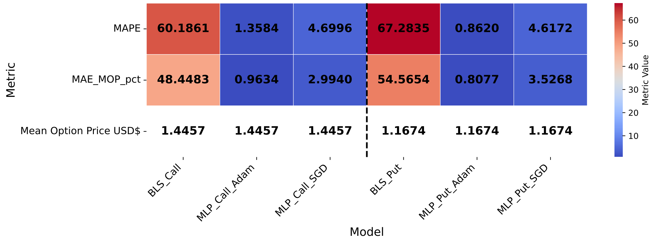
Black-Scholes (BLS) vs MLP 8L 3600N (Adam & SGD) — TRAIN GLD (2010-2015) — MAPE & MAE/MOP %
