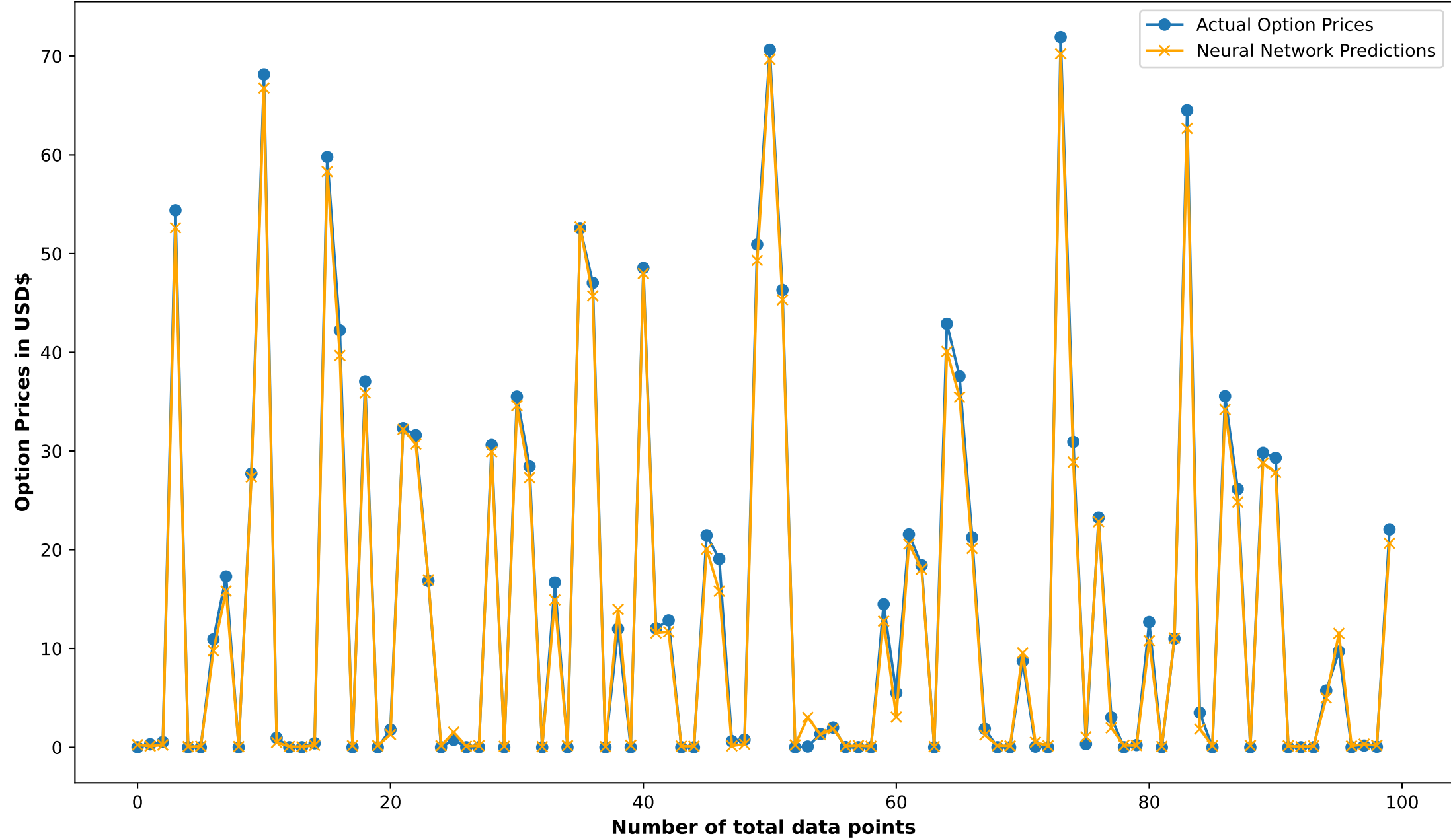
Project 1. Actual Call Option Price vs Neural Network Predictions, Baseline ANN - 3L 150N, SGD optimizer, 1035 point training set, 100 point test set without momentum
