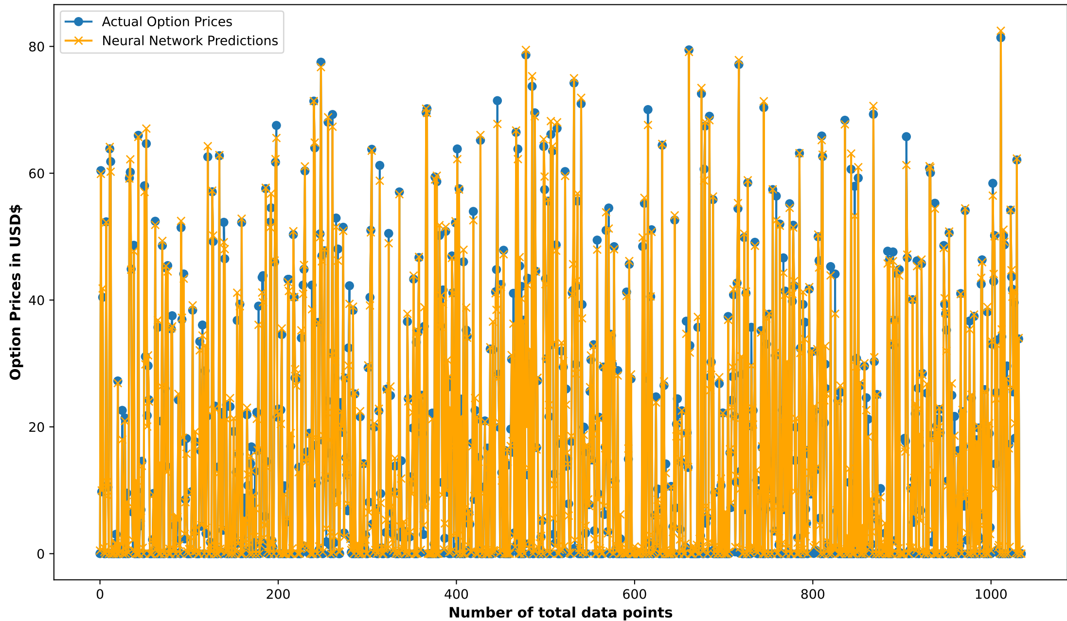
Project 1. Actual Call Option Price vs Neural Network Predictions, "Expanded" ANN - 7L 700N, SGD optimizer, 1035 point training set
