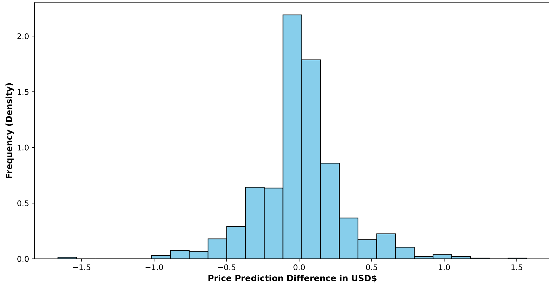
Project 1. Histogram of Prediction Differences "Baseline" ANN - 3L 150N, SGD optimizer, 1035 point training set with momentum
