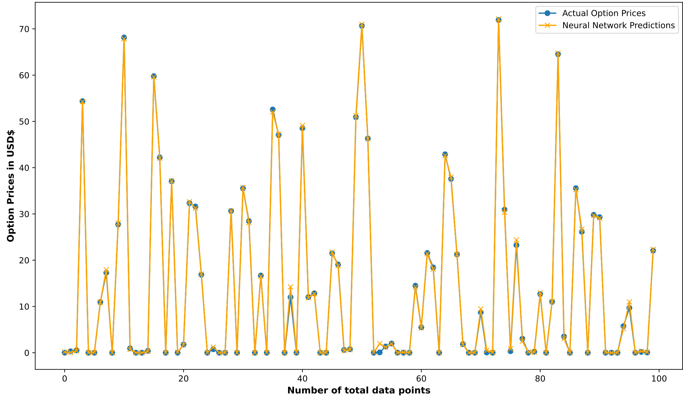
Project 1. Actual Call Option Price vs Neural Network Predictions, Baseline ANN - 3L 150N, SGD optimizer, 1035 point training set, 100 point test set with momentum
