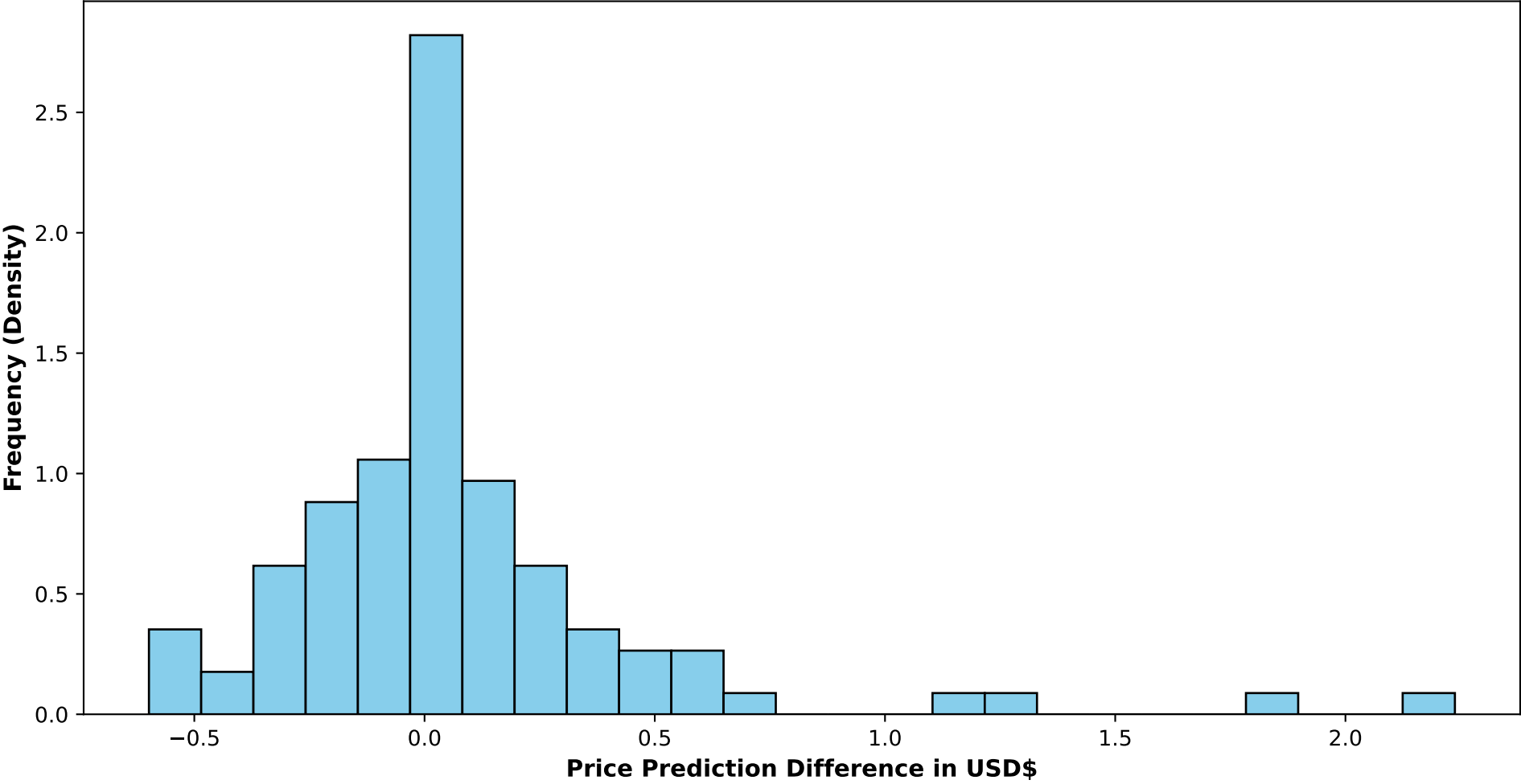
Project 1. Histogram of Prediction Differences Baseline ANN -3L 150N, SGD optimizer, 1035 point training set, 100 point test set with momentum
