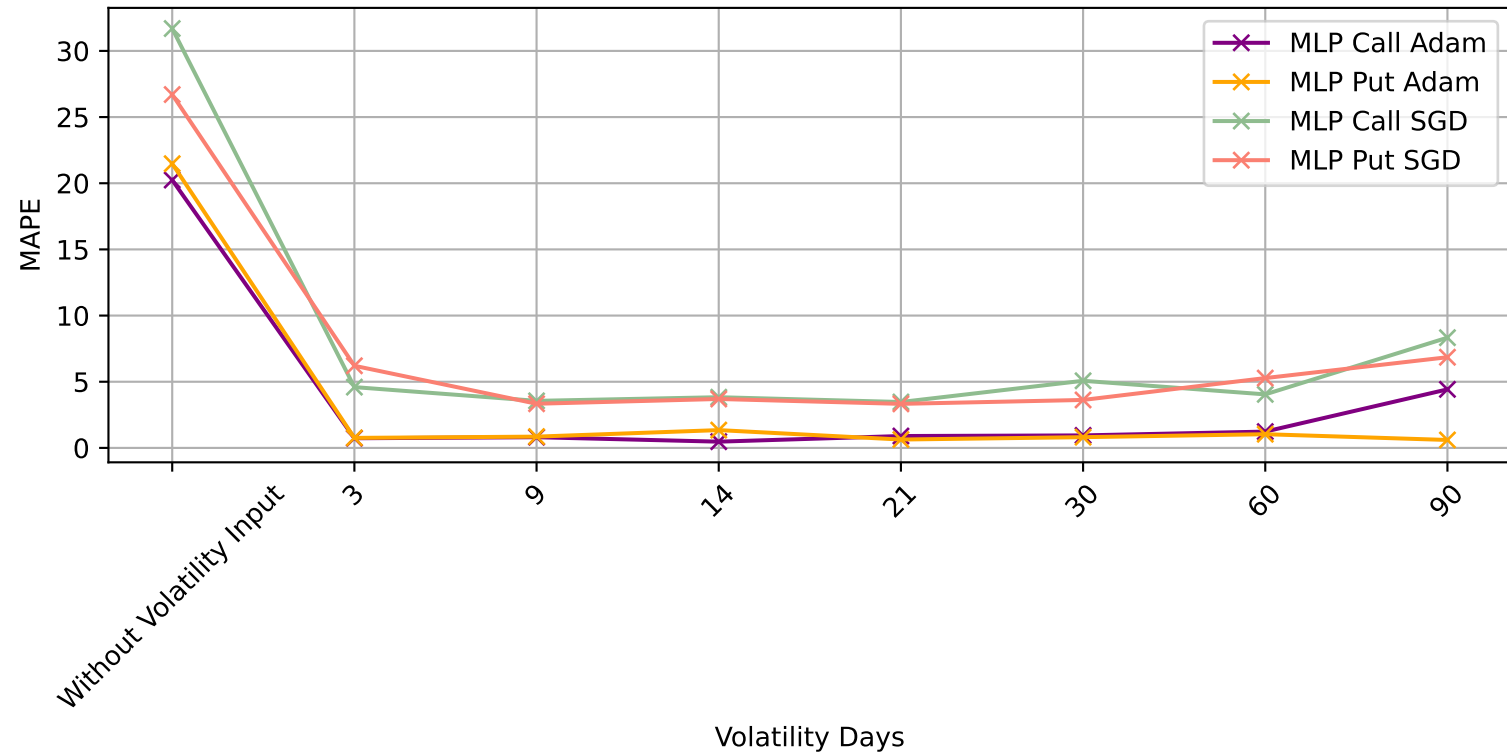
Testing — MLP MAPE
