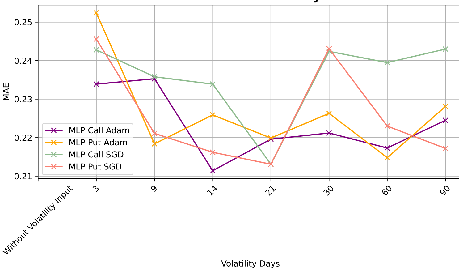
MLP MAE vs Volatility
