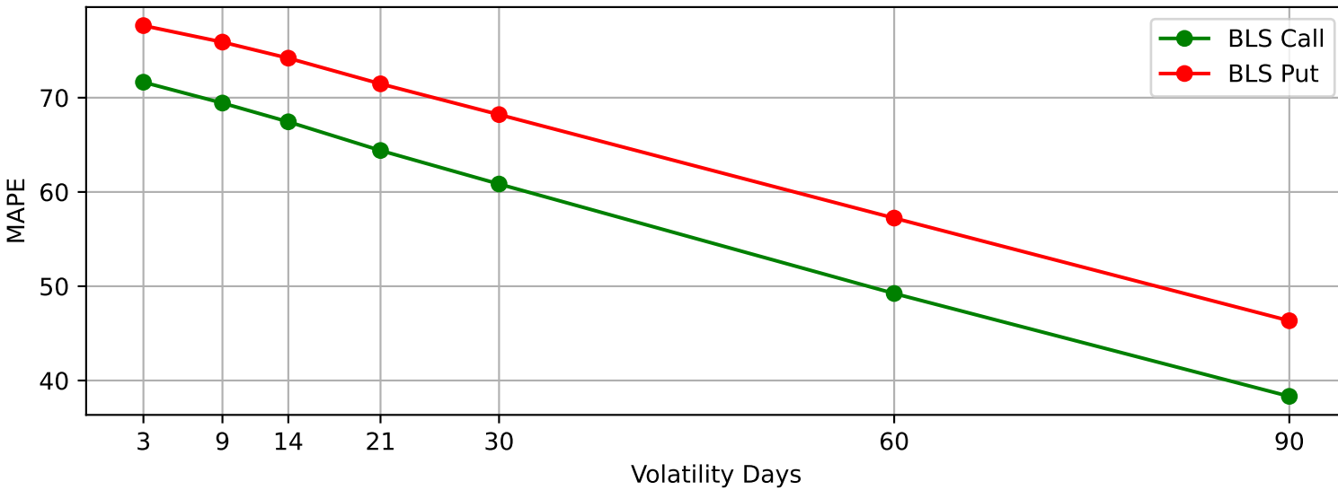
Training — BLS MAPE
