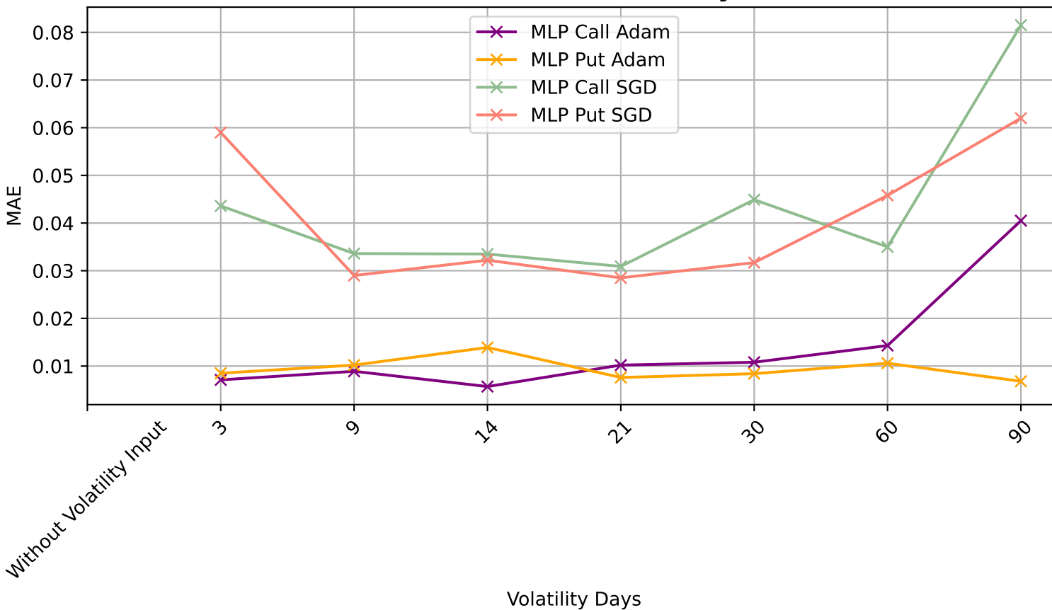
MLP MAE vs Volatility
