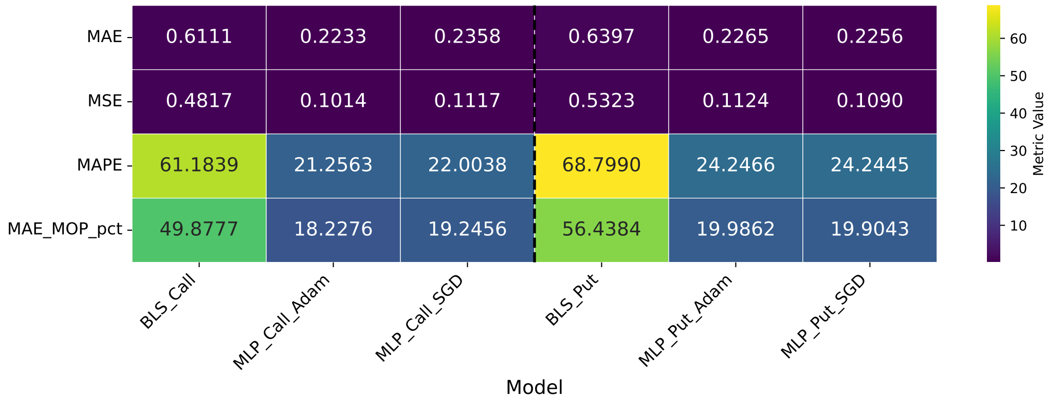
BLS vs MLP 8L 3600N (Adam & SGD) — TEST (2016-2017) — Mean Metrics CALL & PUT
