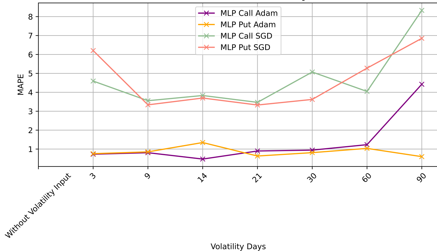
MLP MAPE vs Volatility
