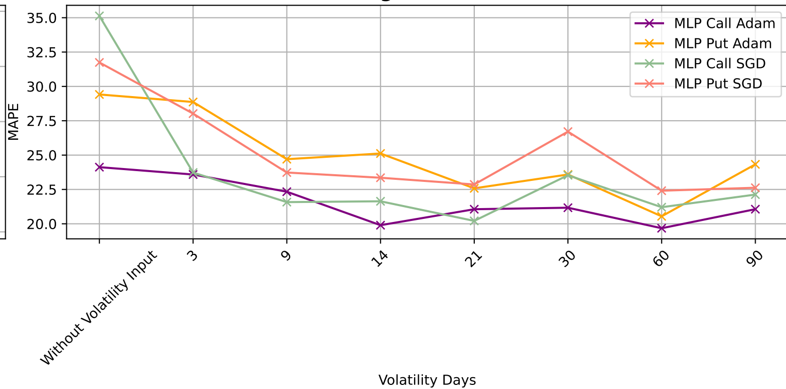
Testing — MLP MAPE
