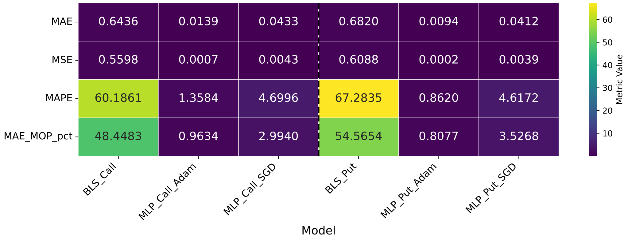
BLS vs MLP 8L 3600N (Adam & SGD) — TRAIN (2010-2015) — Mean Metrics CALL & PUT
