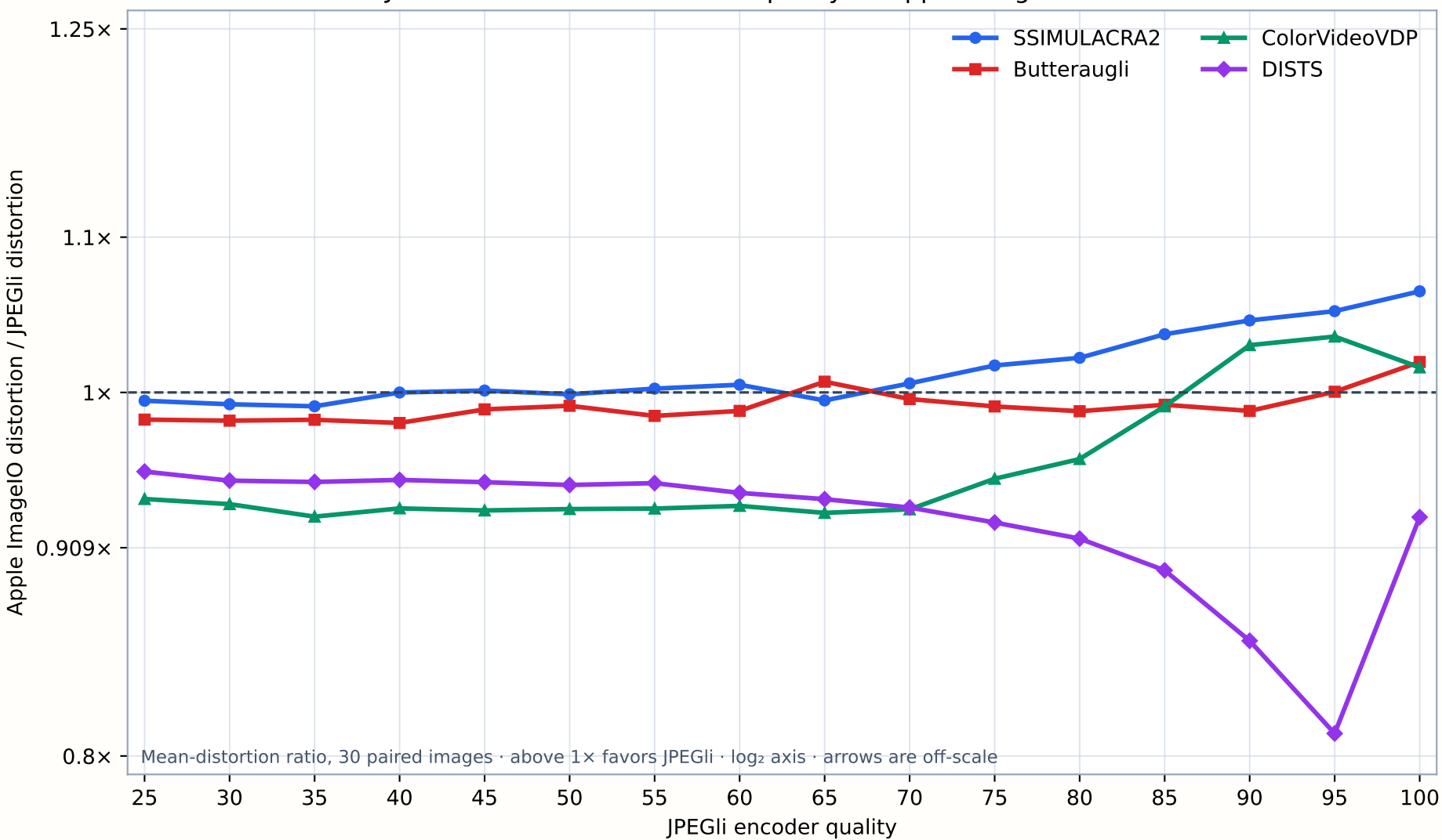
JPEGli relative reconstruction quality vs Apple ImageIO — 4:2:0
