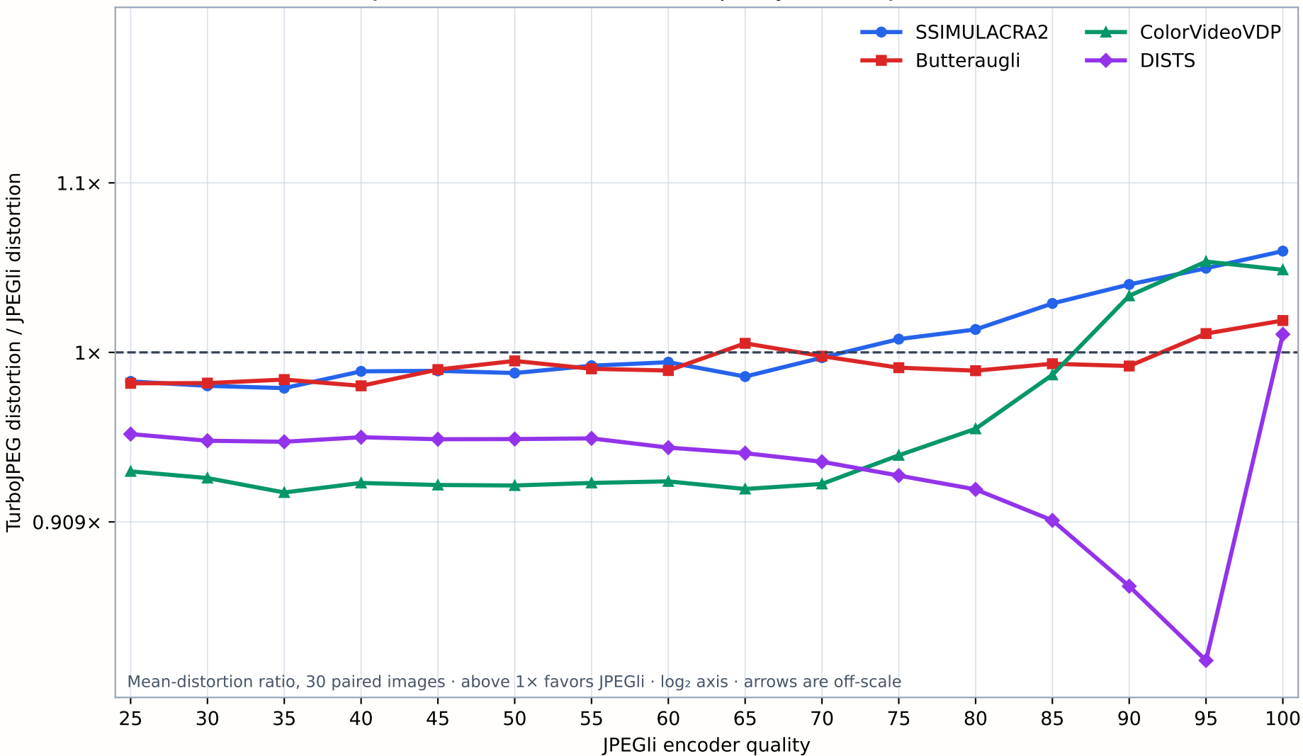
JPEGli relative reconstruction quality vs TurboJPEG — 4:2:0
