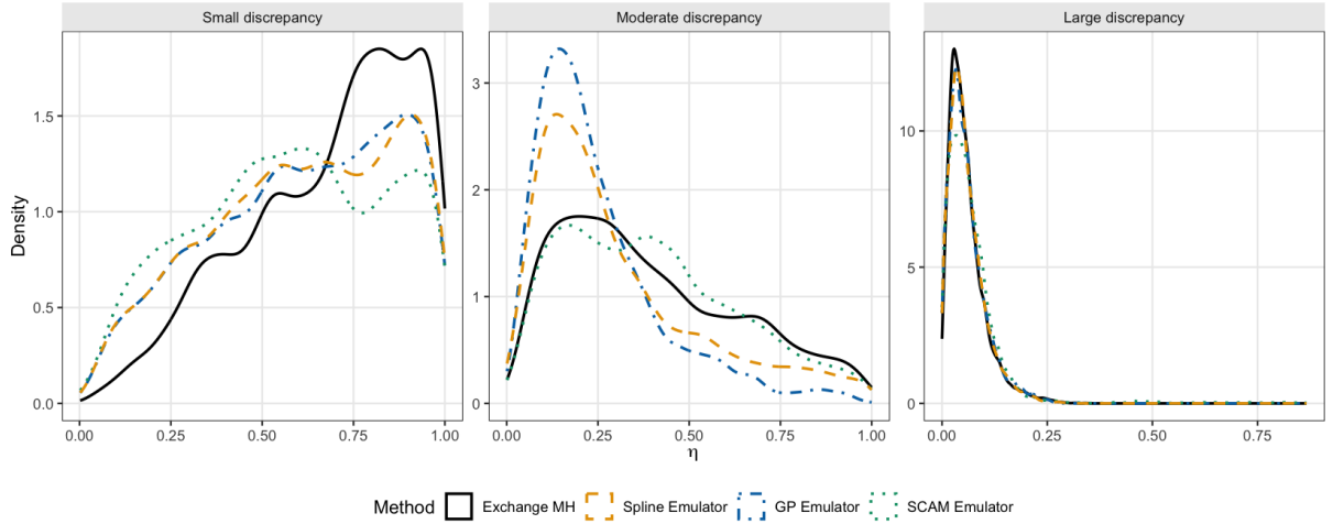
Figure 6 – Posterior density of \eta across discrepancy scenarios for the logistic regression normalised power prior experiment.
