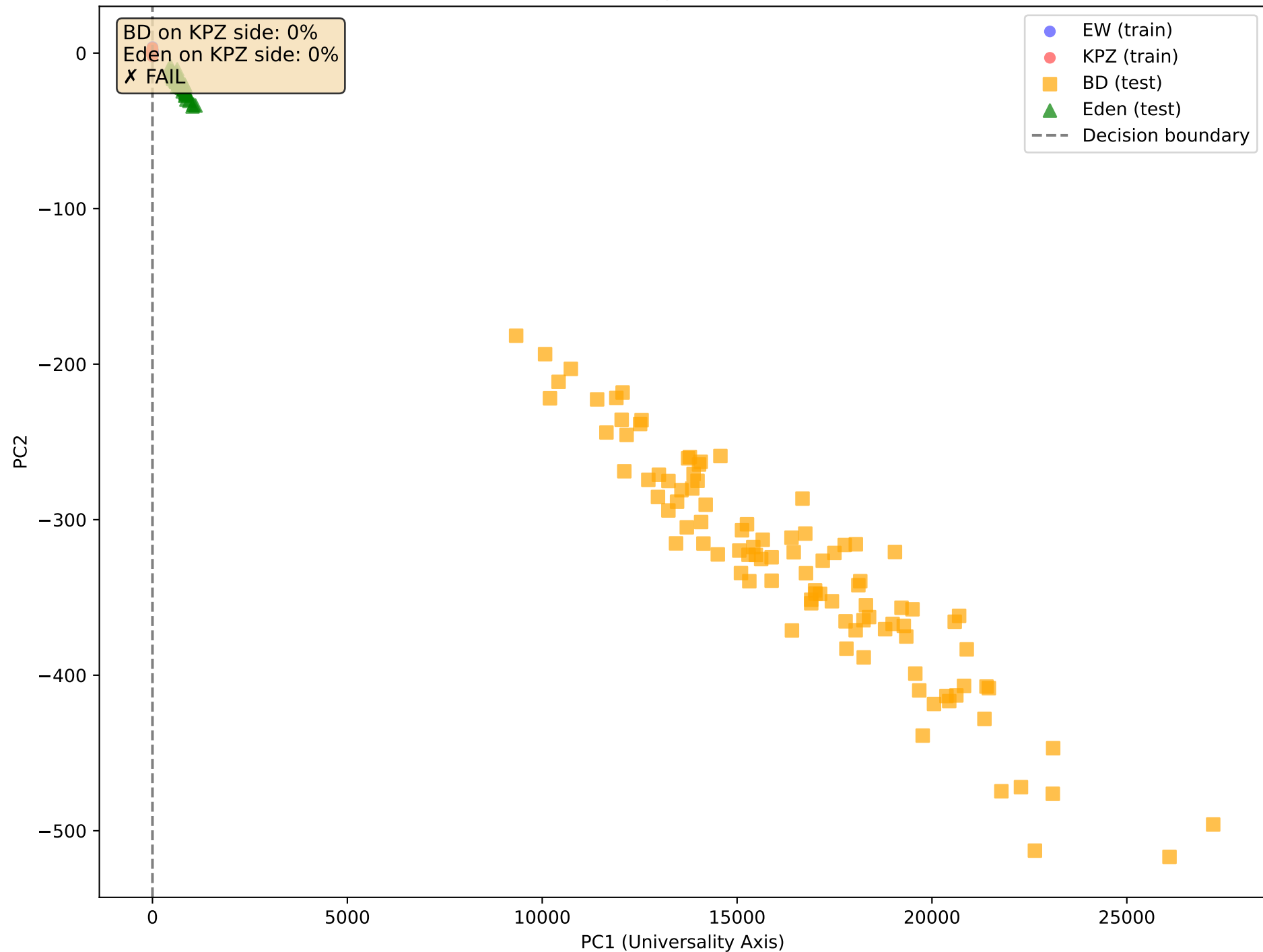
TEST 1: Do BD/Eden land on KPZ side? (PCA fit only on EW+KPZ)
