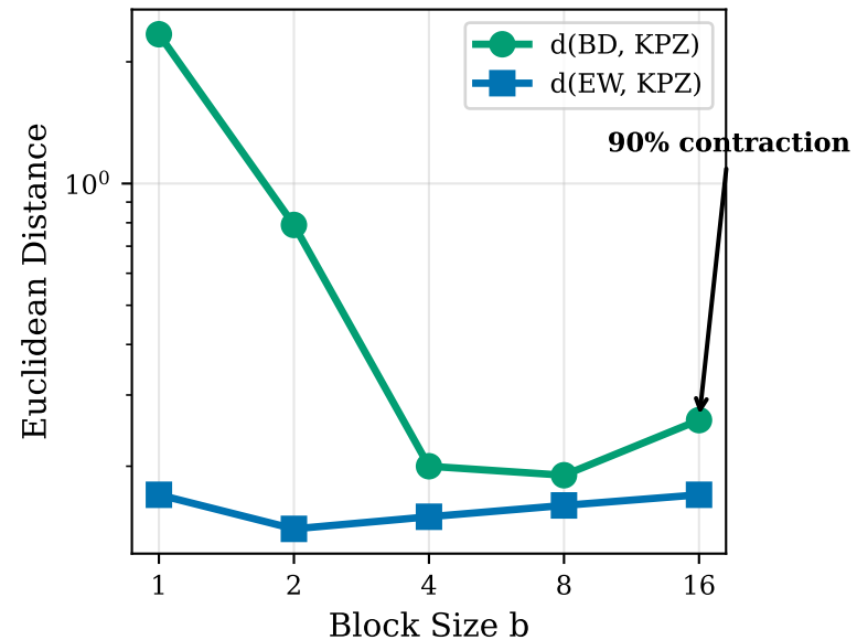
(A) RG Flow: BD→KPZ Convergence
