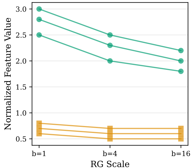
(C) Feature Convergence
