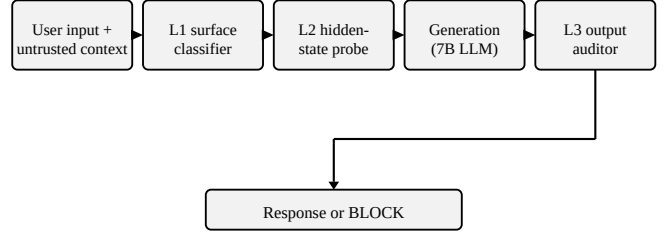
Fig. 1. The three-layer pipeline. L2 runs on every input L1 does not hard-block (“always-on” routing); L3 audits the generated output. Any layer can block the request, fail-closed.
