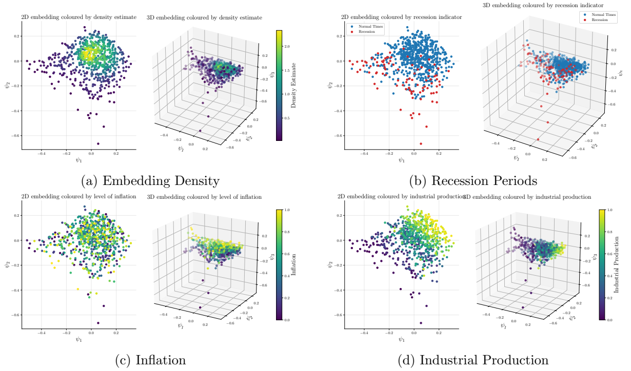
Figure 2: Diffusion-map representation of the quantile-transformed macroeconomic observations using \alpha = 1 , \varepsilon = 3 . While our diffusion dimension is 4-dimensional, here we only show 2D and 3D plots. Observations are coloured by density, NBER recession labels, inflation rates (quantile), and industrial production levels (quantile).
