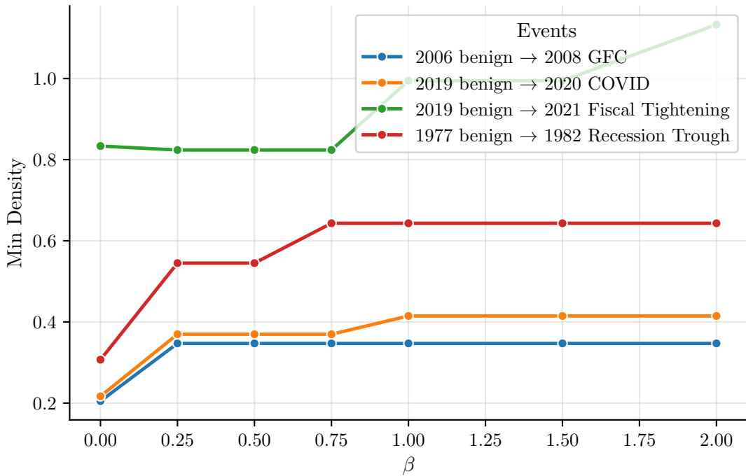
Interior Minimum Density vs. \beta by Event
