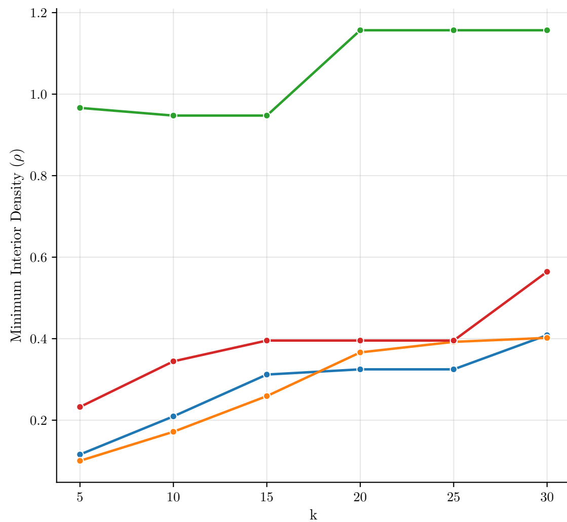
Latent path metrics against a changing number of nearest neighbours in graph construction
