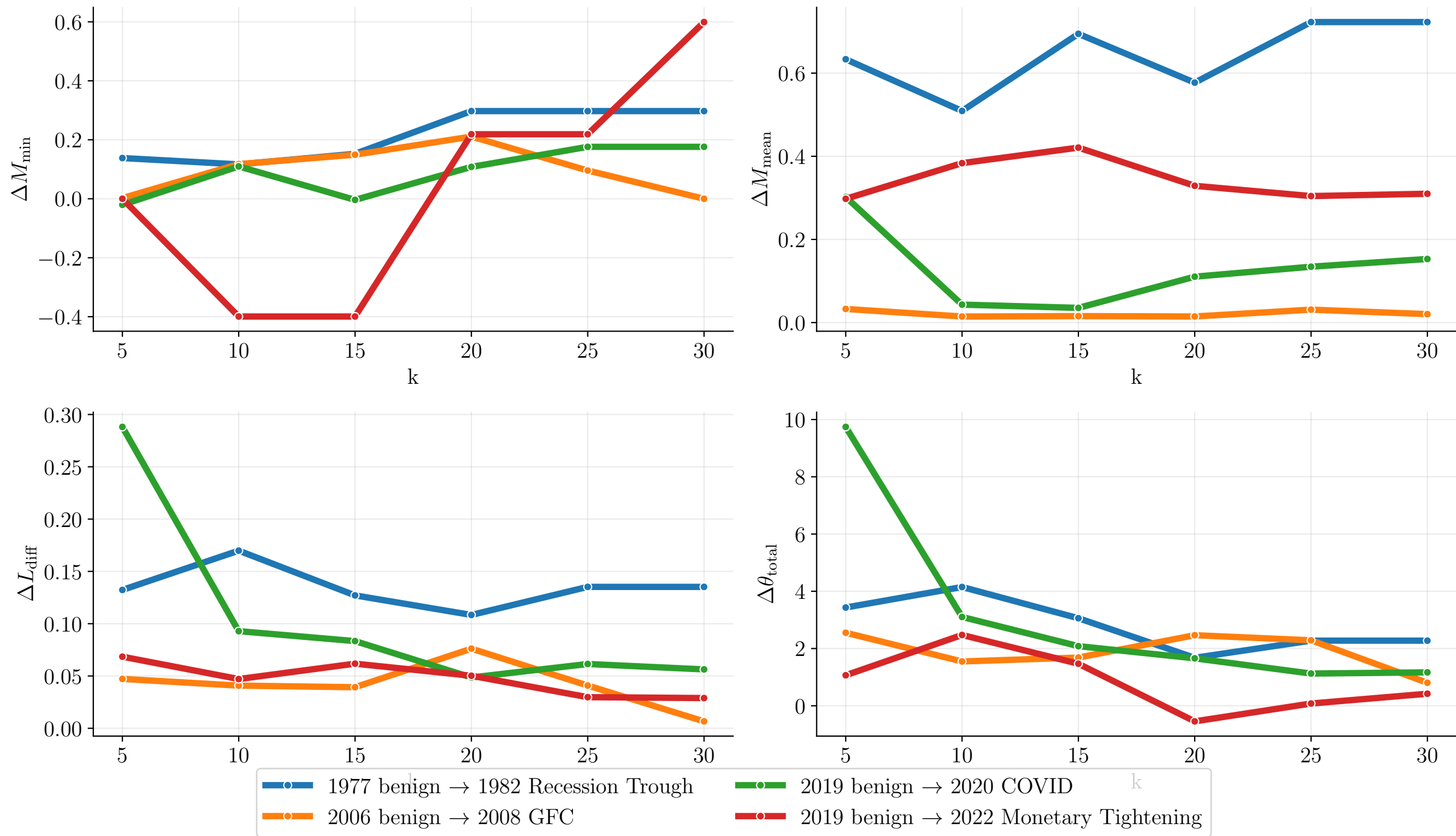
Latent path metrics against a changing number of nearest neighbours in graph construction
