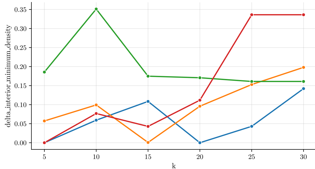
Latent path metrics against a changing number of nearest neighbours in graph construction
