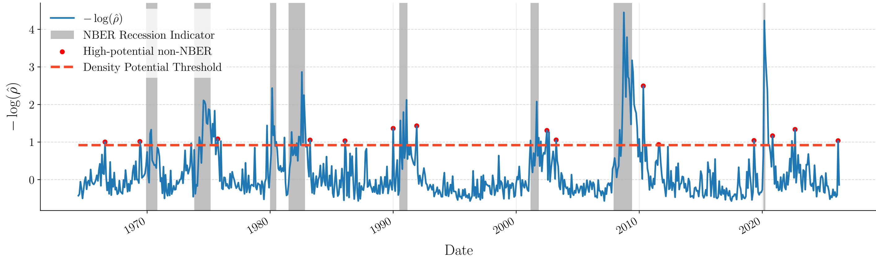
Embedding Density Potential vs. NBER Recession Periods
