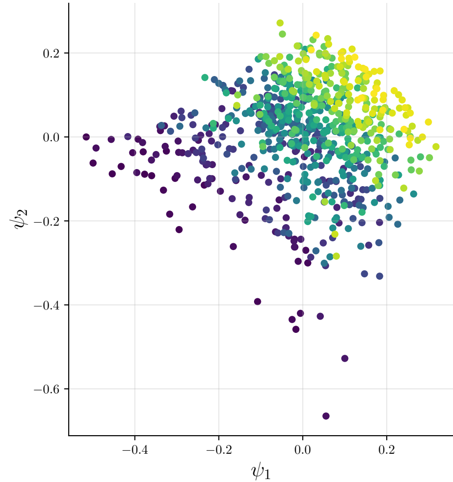
2D embedding coloured by industrial production
