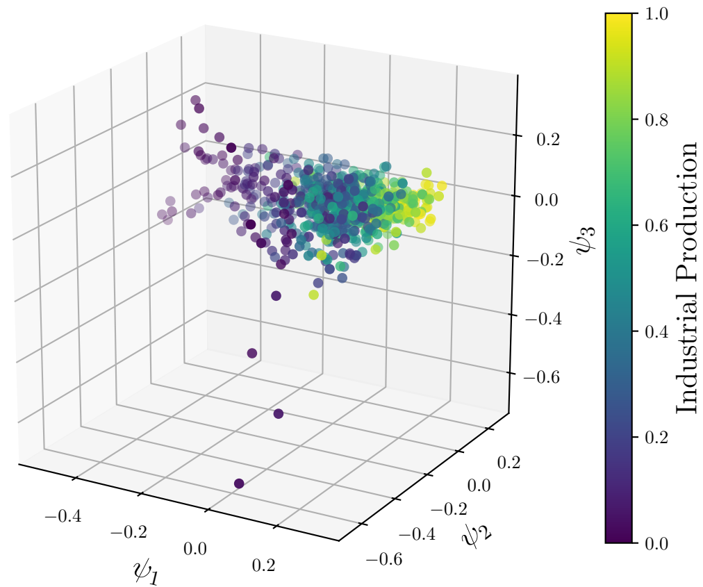
3D embedding coloured by industrial production
