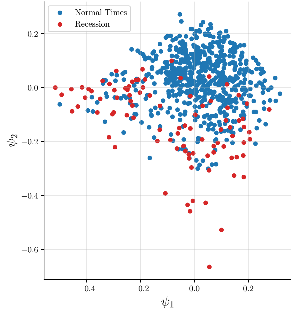
2D embedding coloured by recession indicator
