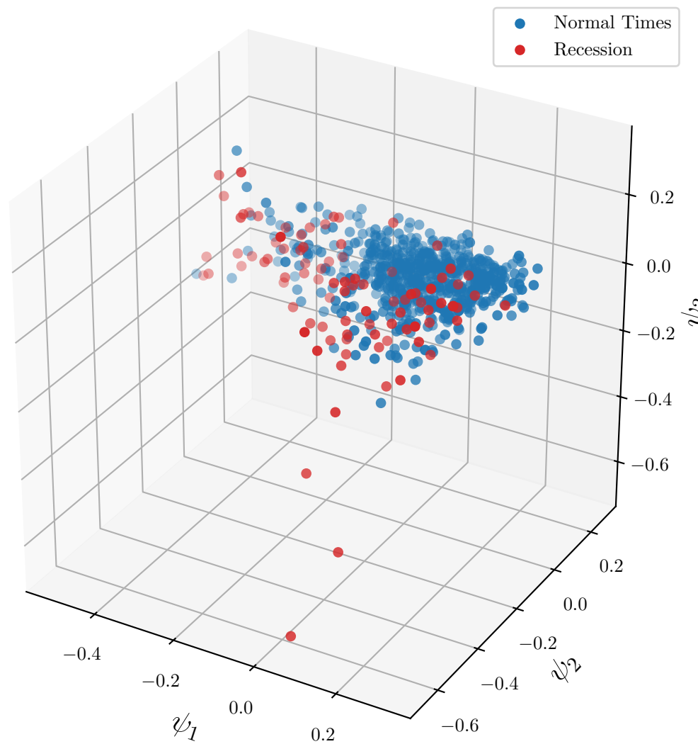
3D embedding coloured by recession indicator
