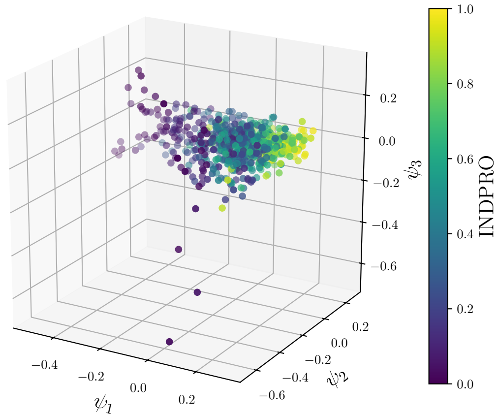
3D embedding coloured by INDPRO (Quantile)
