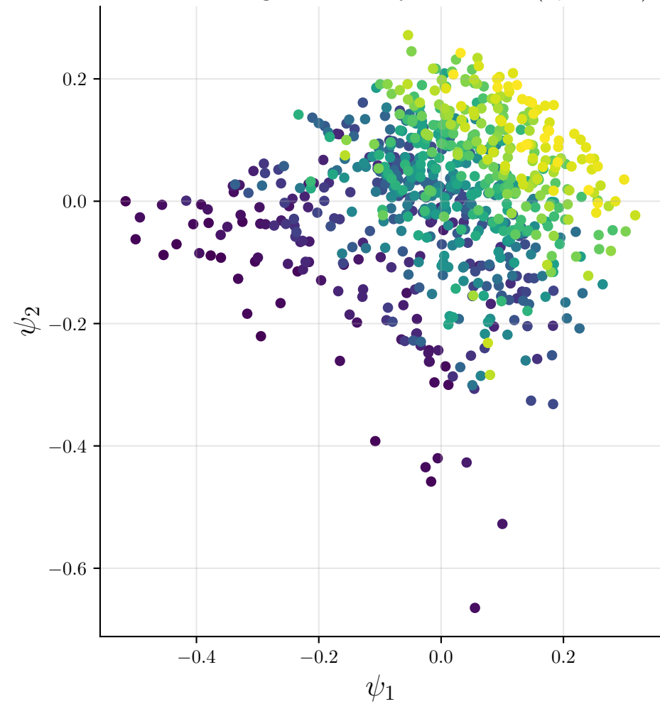
2D embedding coloured by INDPRO (Quantile)
