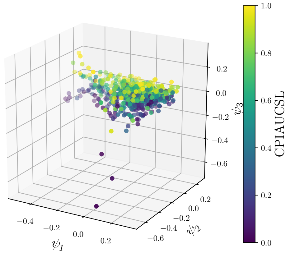
3D embedding coloured by CPIAUCSL (Quantile)
