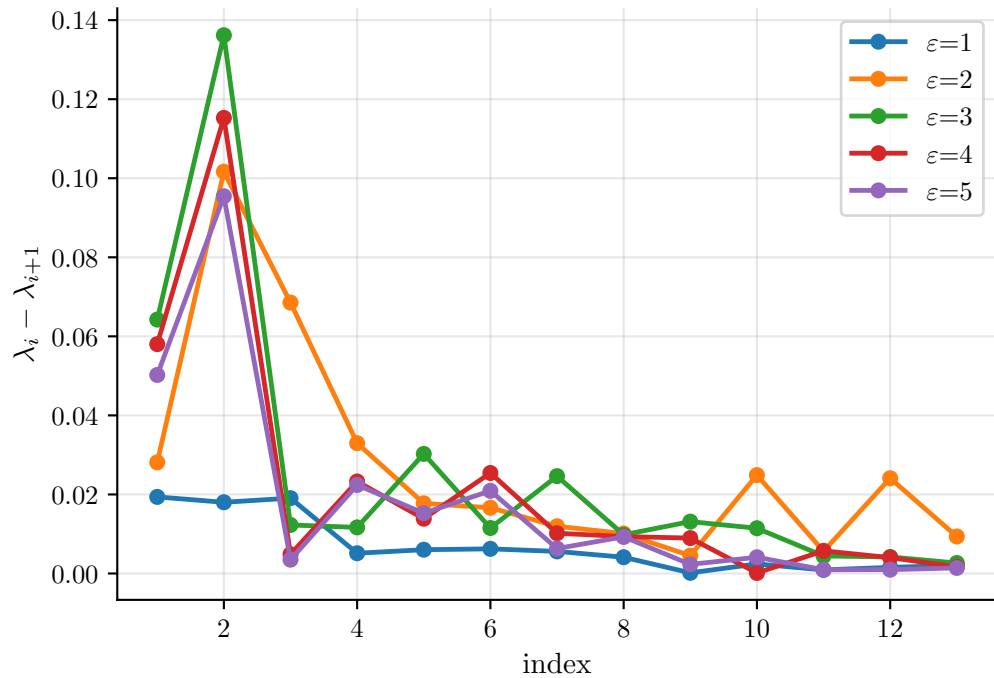
Gaps between eigenvalues for different levels of \varepsilon
