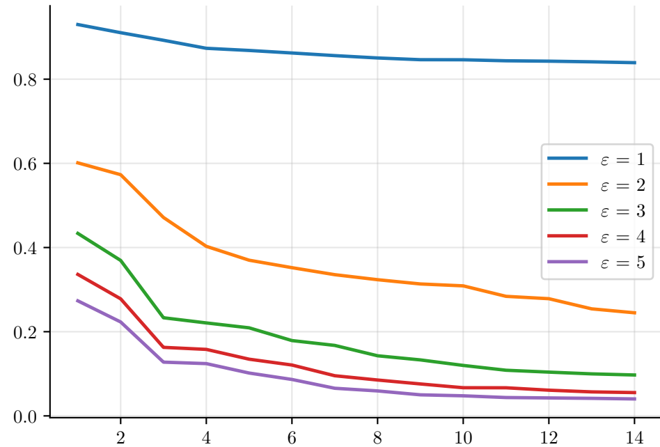
First 14 eigenvalues of transition matrix for different levels of \varepsilon
