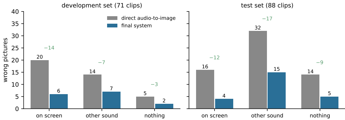
Figure 4: Wrong pictures by kind (Section 3.3), direct audio-to-image generation against the final system. Green: the number removed. Totals: 39 \rightarrow 15 (development), 62 \rightarrow 24 (test). The on-screen check removes on-screen pictures directly; silencing a sound also removes its late repeats (other sound), and the depict-event check removes some more. On the test set 17 of the 38 removed pictures are of another sound and 9 of nothing.
