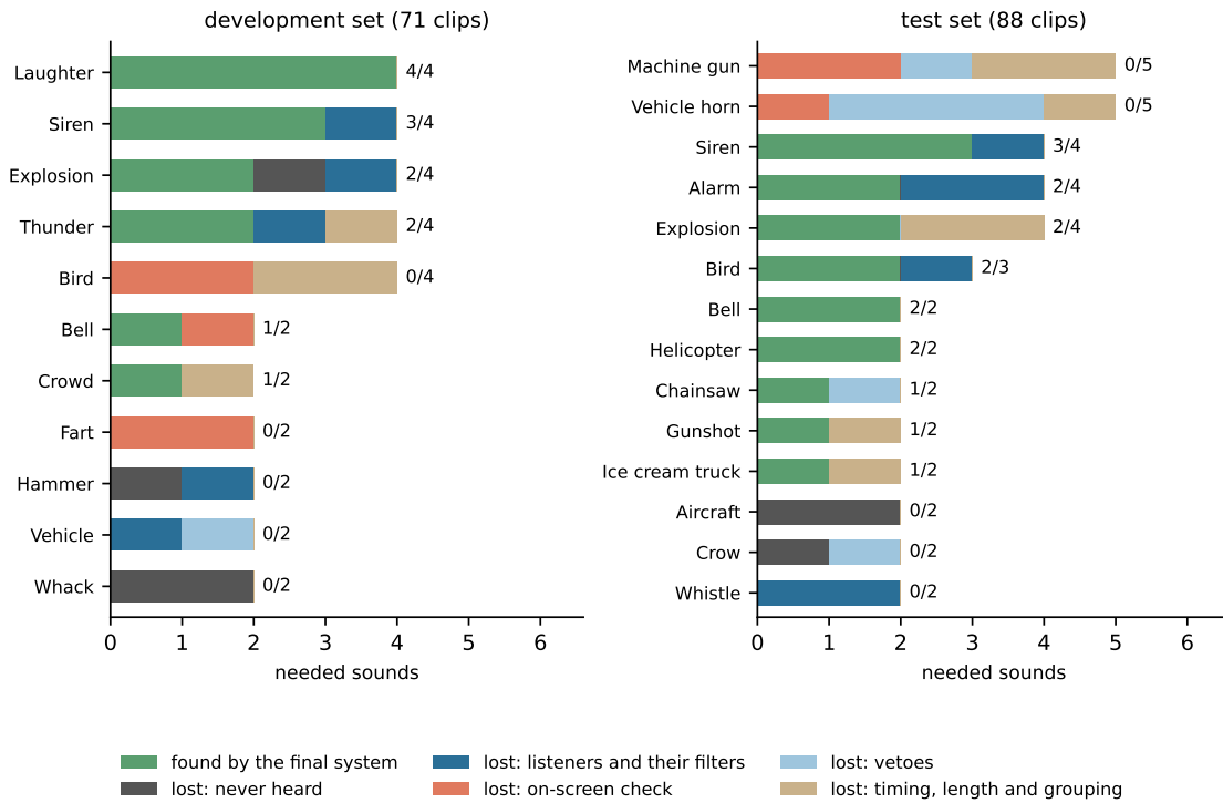
Figure 9: Needed sounds found by the final system, by gold label, for every label with at least two needed sounds in that set. Green: found; the rest of each bar is stacked by the step where the sound was lost, in the colours of Figure 8. Per-sound outcomes from the logged decision trail ( docs/decision_trail/data.js ).
