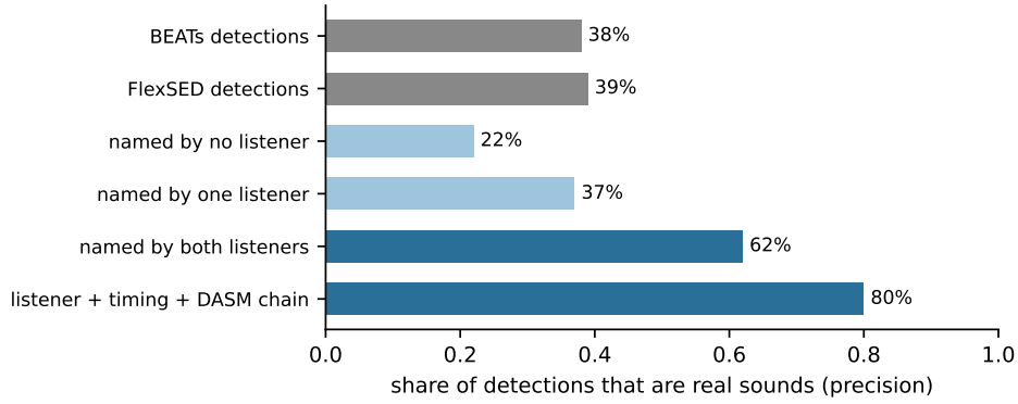
Figure 8: Share of detections that are real sounds, on the screening set (415 AudioSet-Strong clips with timed labels). Raw detections are right less than 40 % of the time; agreement between models helps, but a sound only one listener names is right just over a third of the time.
