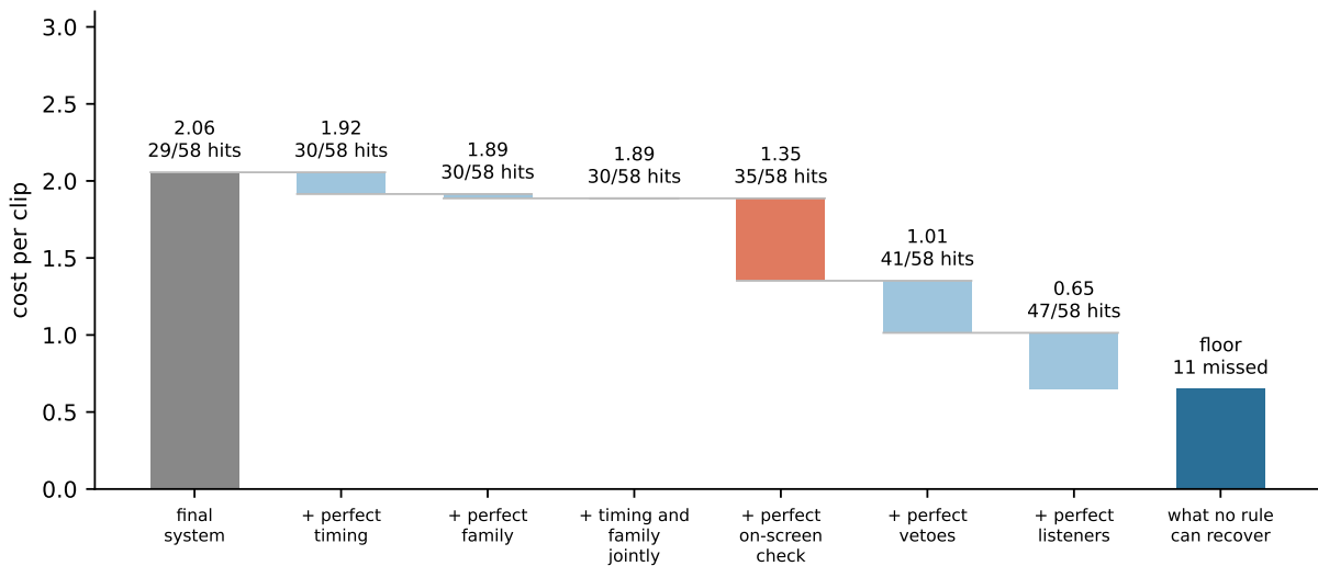
Figure 13: Ceiling analysis of the final system (development set, 58 needed sounds). Each bar makes one more stage perfect, using the labels, on the same detections. The largest single step, the on-screen check, is shown in red. Even with every stage perfect, 11 needed sounds remain missed (right): the detectors never hear them clearly enough.
