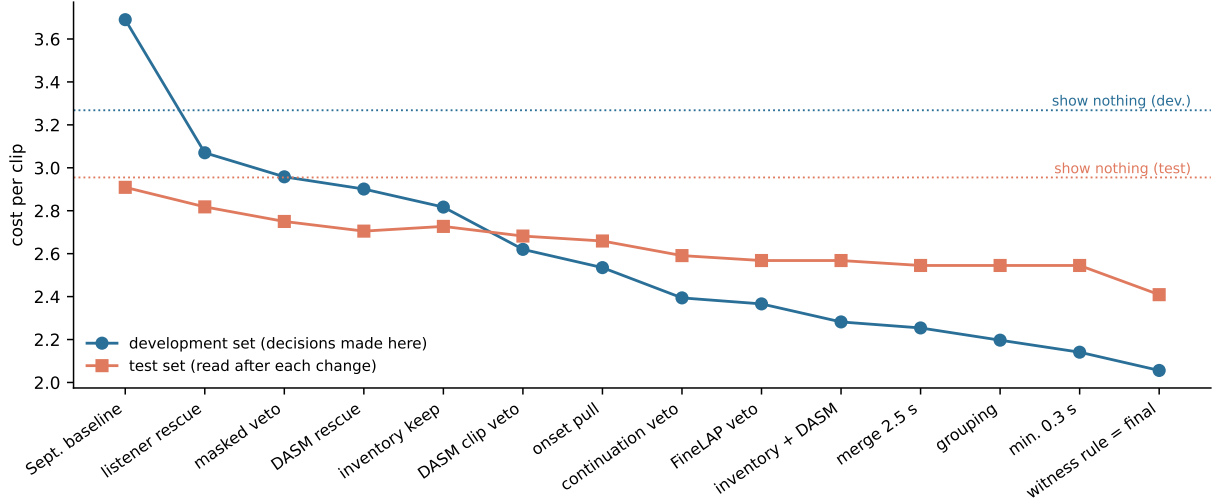
Figure 9: Cost per clip after each accepted change. Decisions were made on the development set; the test set was read after each change and only reported. Dotted lines: showing nothing.
