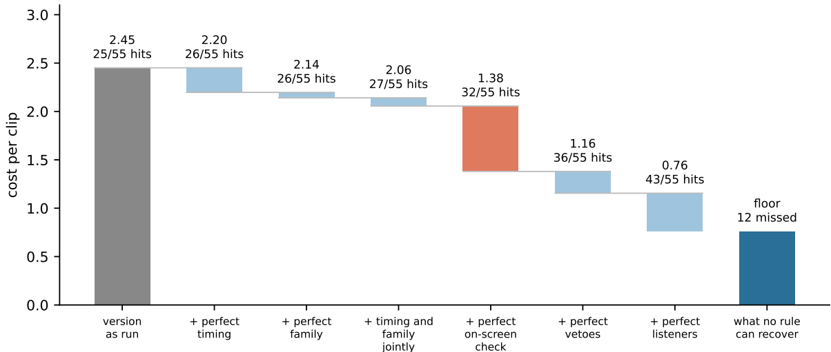
Figure 13: Ceiling analysis on a slightly older version of the system (development set, 55 needed sounds). Each bar makes one more stage perfect, using the labels, on the same detections. The 2.06 after the joint timing and family step equals the final system’s development cost only by coincidence. The largest single step, the on-screen check, is shown in red. Even with every stage perfect, 12 needed sounds remain missed (right): the detectors never hear them clearly enough.
