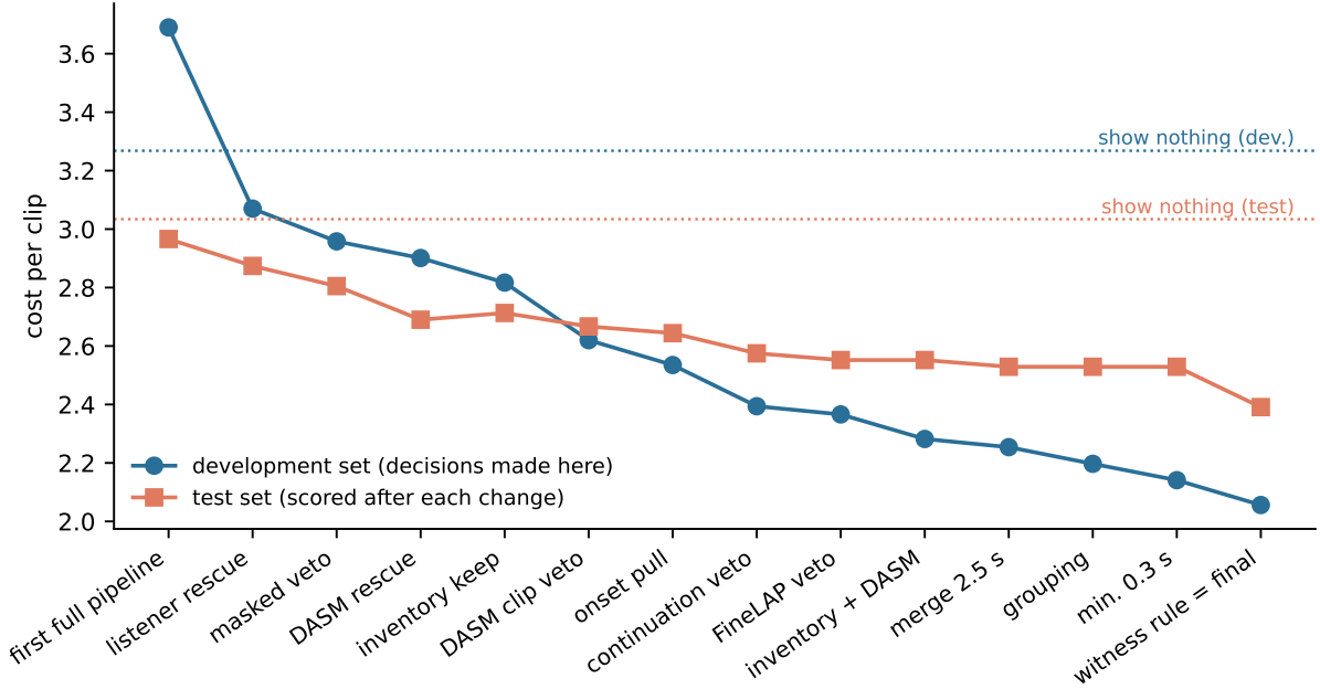
Figure 11: Cost per clip after each accepted change, from the first full pipeline to the final system: development 3.690 → 2.056, test 2.966 → 2.391. Decisions were made on the development set; the test set was only scored. Dotted lines: showing nothing. Each step is a row of Table 15 (Appendix E), except three early steps (masked-weak veto, DASM rescue, inventory keep), which share one row there. The depict-event row (net effect zero) and the row in which the scene check is read as text instead of as a probability (Appendix E.10) are not plotted. The step names are short forms of the internal names explained in Appendix D.
