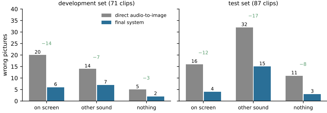
Figure 4: Wrong pictures by kind (Section 3.3), direct audio-to-image generation against the final system. Green: the number removed. Totals: 39 → 15 (development), 59 → 22 (test). The on-screen check removes on-screen pictures directly; silencing a sound also removes its late repeats (other sound), and the depict-event check removes some more. On the test set 17 of the 37 removed pictures are of another sound and 8 of nothing.
