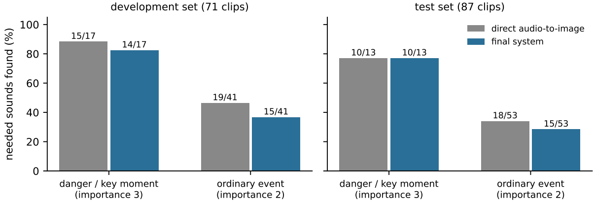
Figure 6: Needed sounds found, by importance level (bars: share found; labels: found / needed). Importance 3: danger or a key moment, such as a siren, an alarm, glass or a baby crying; importance 2: an ordinary event one can say in a sentence. The final system finds 82 % (development) and 77 % (test) of the danger sounds and 37 % and 28 % of the ordinary events; direct audio-to-image finds 88 % and 77 %, and 46 % and 34 %, with far more wrong pictures (Figure 3).
