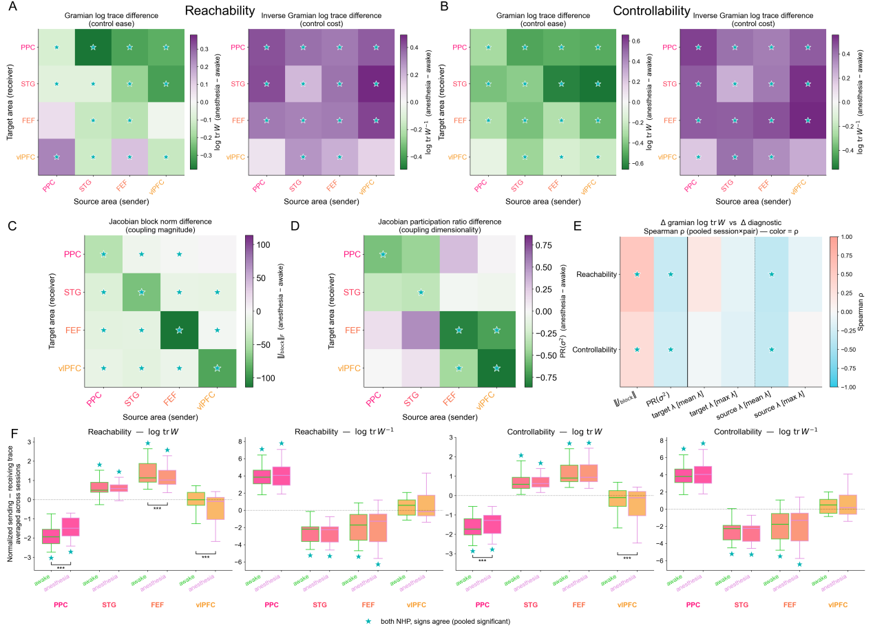
Figure 5. Directional reorganization of interareal control under propofol ( n = 21 sessions). (A) 4×4 source–target heatmaps of pooled anesthesia–awake differences in reachability log tr \mathbf{W} (left) and log tr \mathbf{W}^{-1} (right); stars mark cells passing the sign-agree + BH-FDR gate at q < 0.05 . (B) Same for controllability. (C) Jacobian block Frobenius-norm differences. (D) Block participation-ratio differences. (E) Spearman correlation between Gramian-change cells and block-norm/PR-change cells. (F) Per-area net send–receive axis normalized by diagonal within-area measure across all four metrics, placing PPC at the receiver end, FEF/STG at the sender end, vIPFC balanced.
