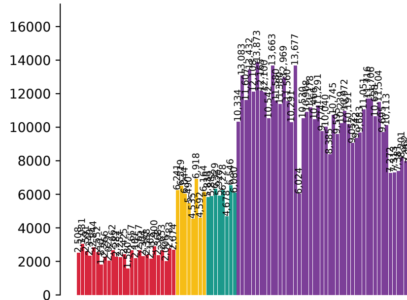
Median sgRNA UMIs/cell
