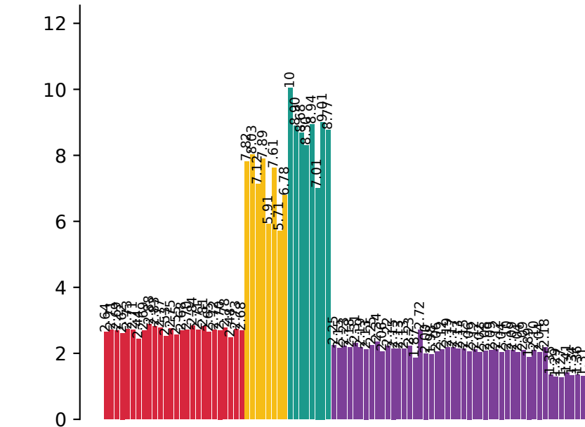
Mean assigned sgRNA/cell
