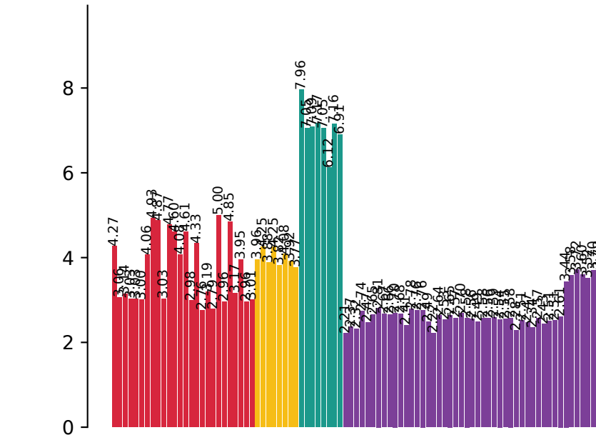
Median Tx % MT UMIs
