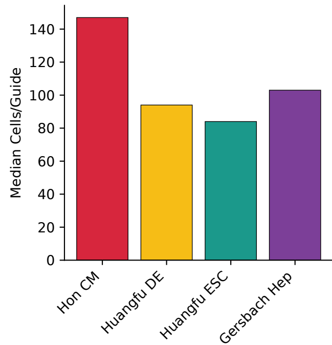
Median Cells/Guide
