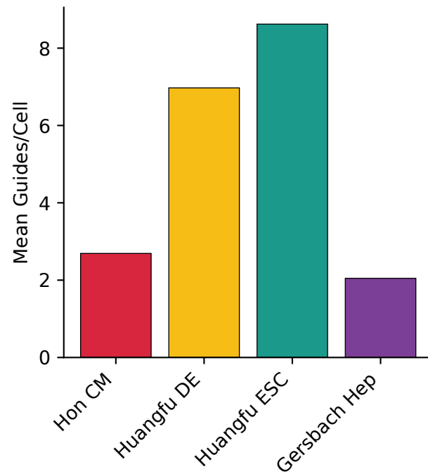
Mean Guides/Cell
