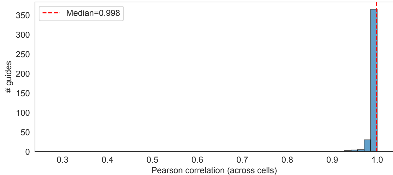
Per-Guide UMI Correlation Distribution
