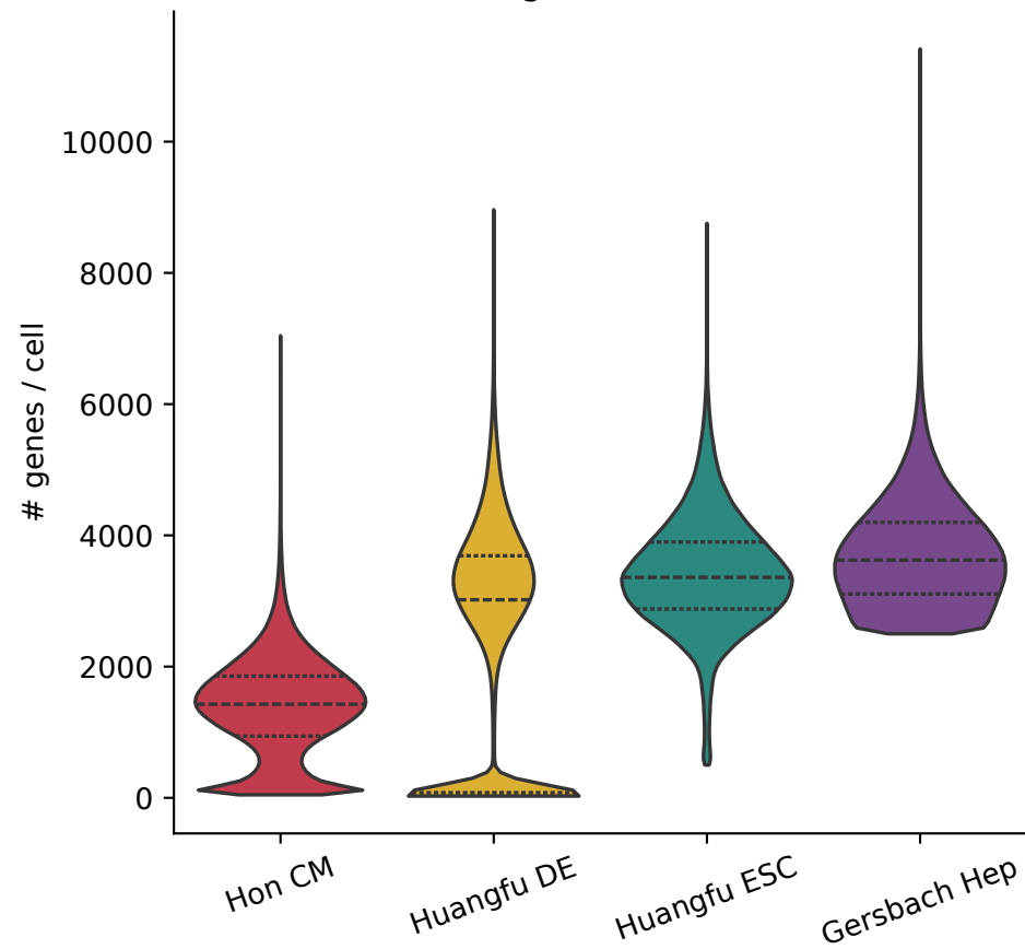
# genes / cell
