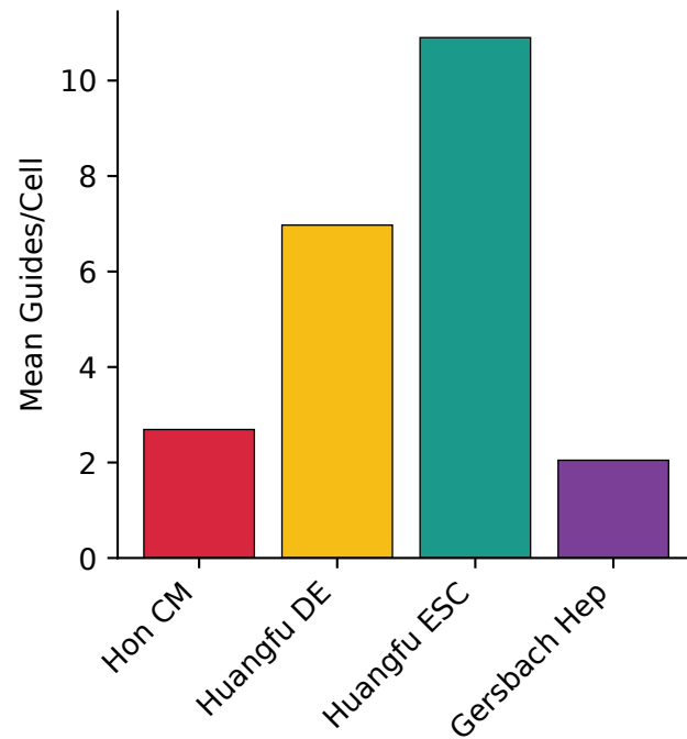
Mean Guides/Cell
