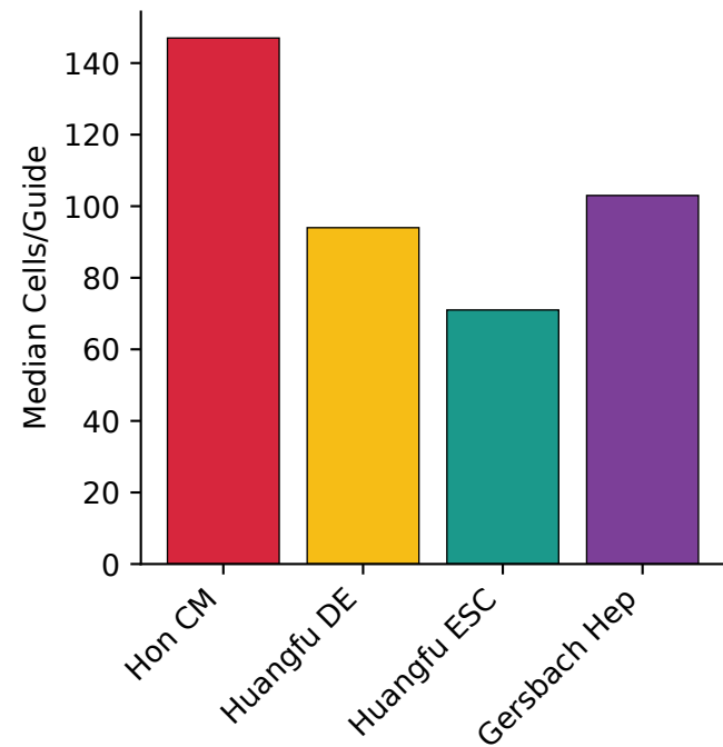
Median Cells/Guide
