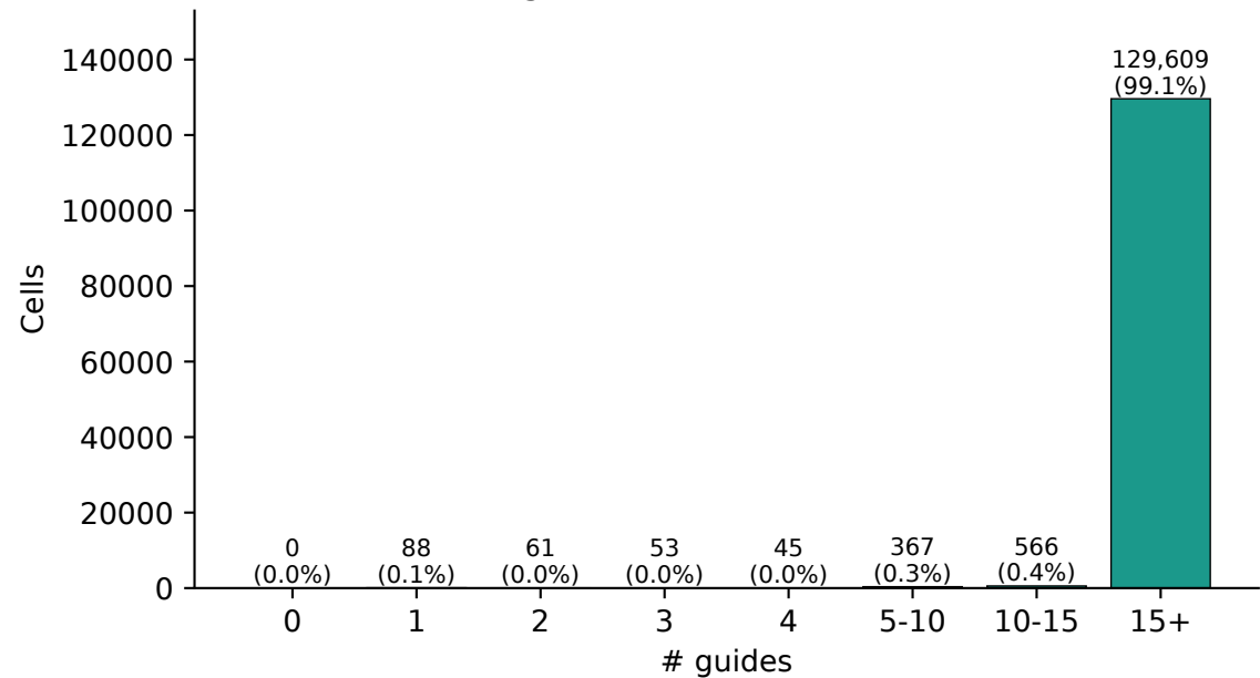
# guides with UMI > 0 / cell
