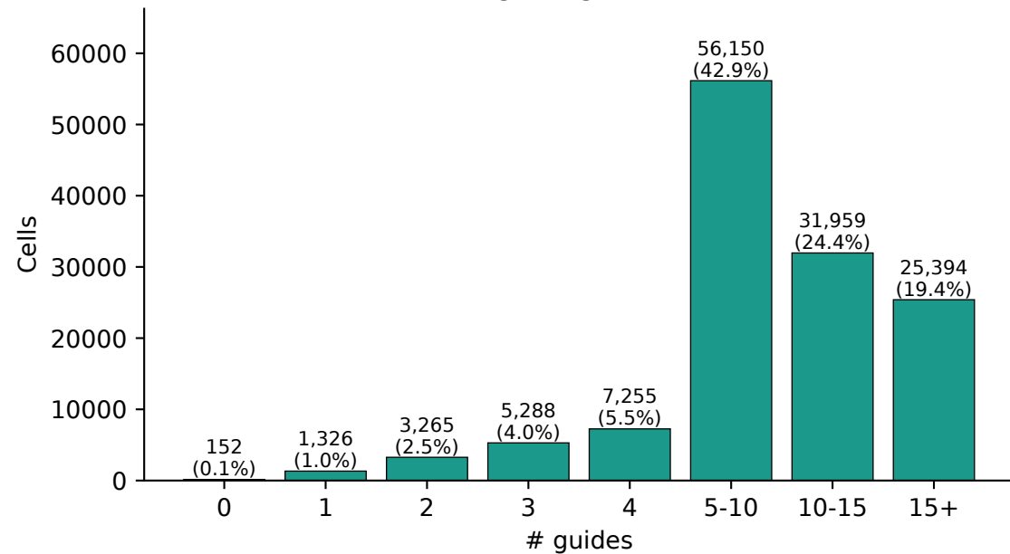
# assigned guides / cell
