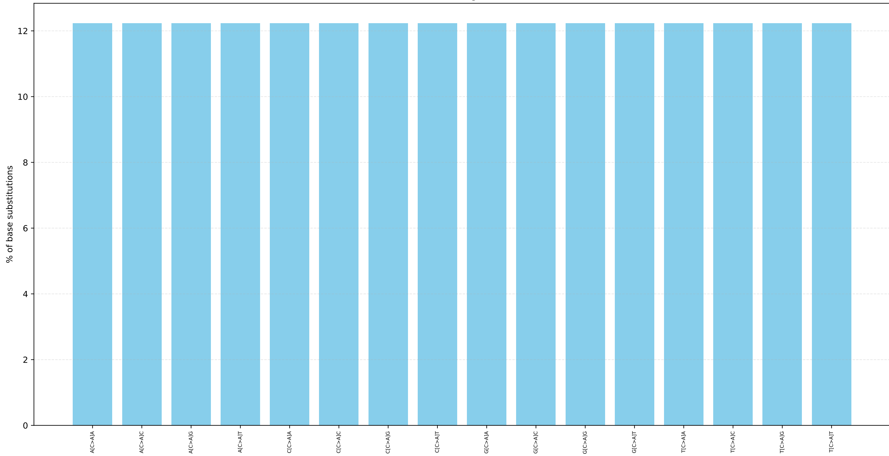
Mutation Signature
