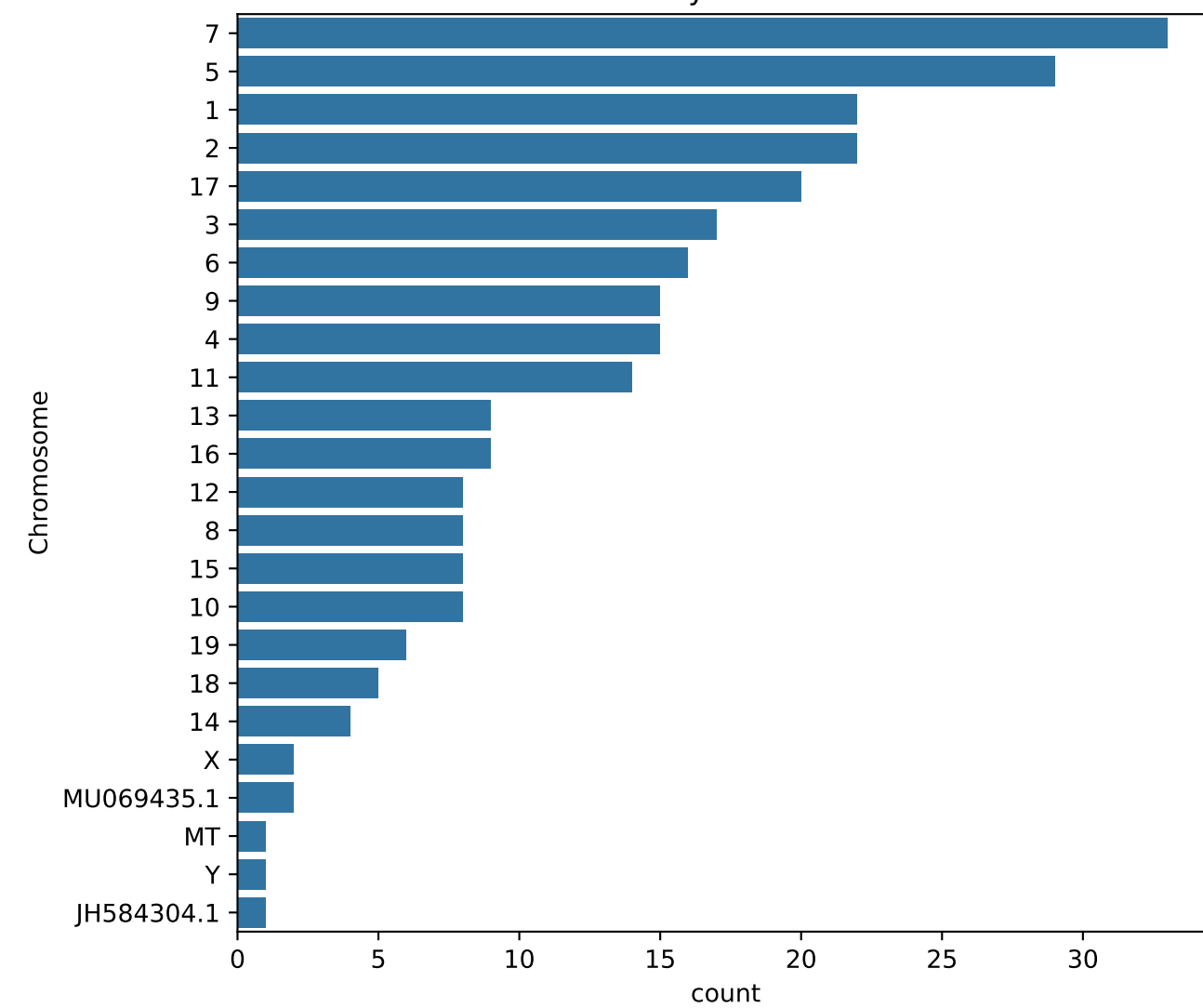
Variants by Chromosome
