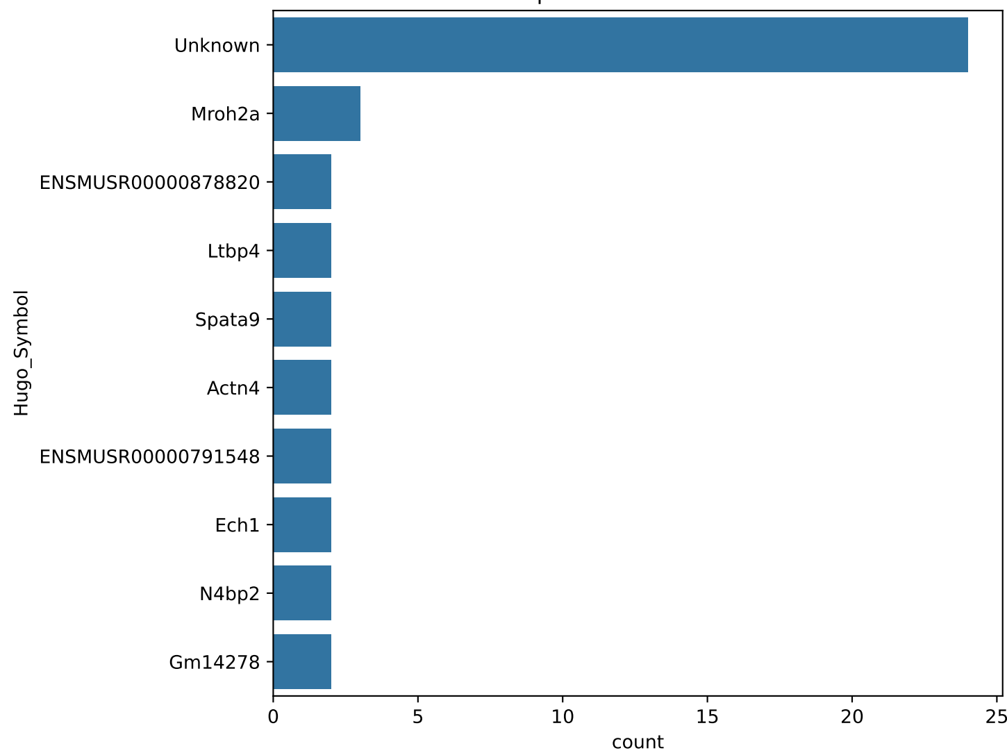
Top 10 Mutated Genes
