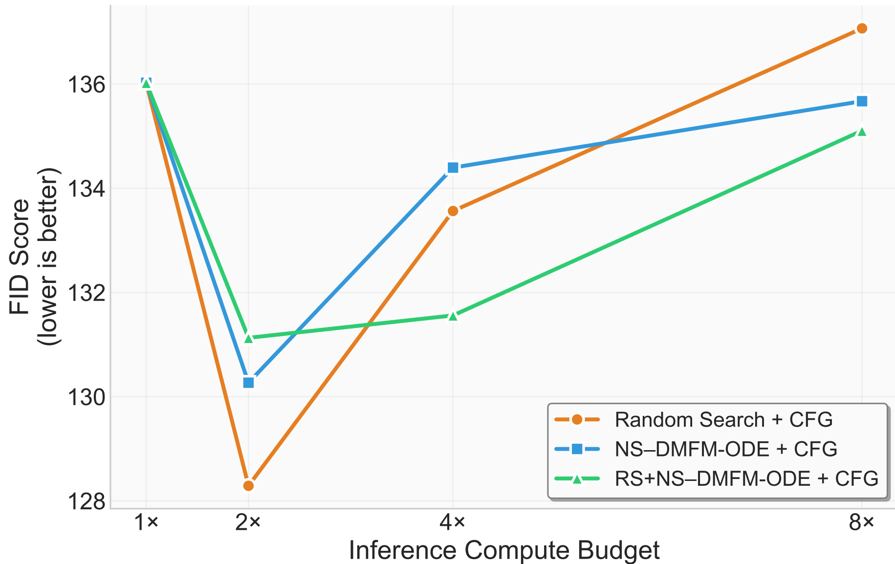
CFG Ablation (scale=1.5): FID Score
