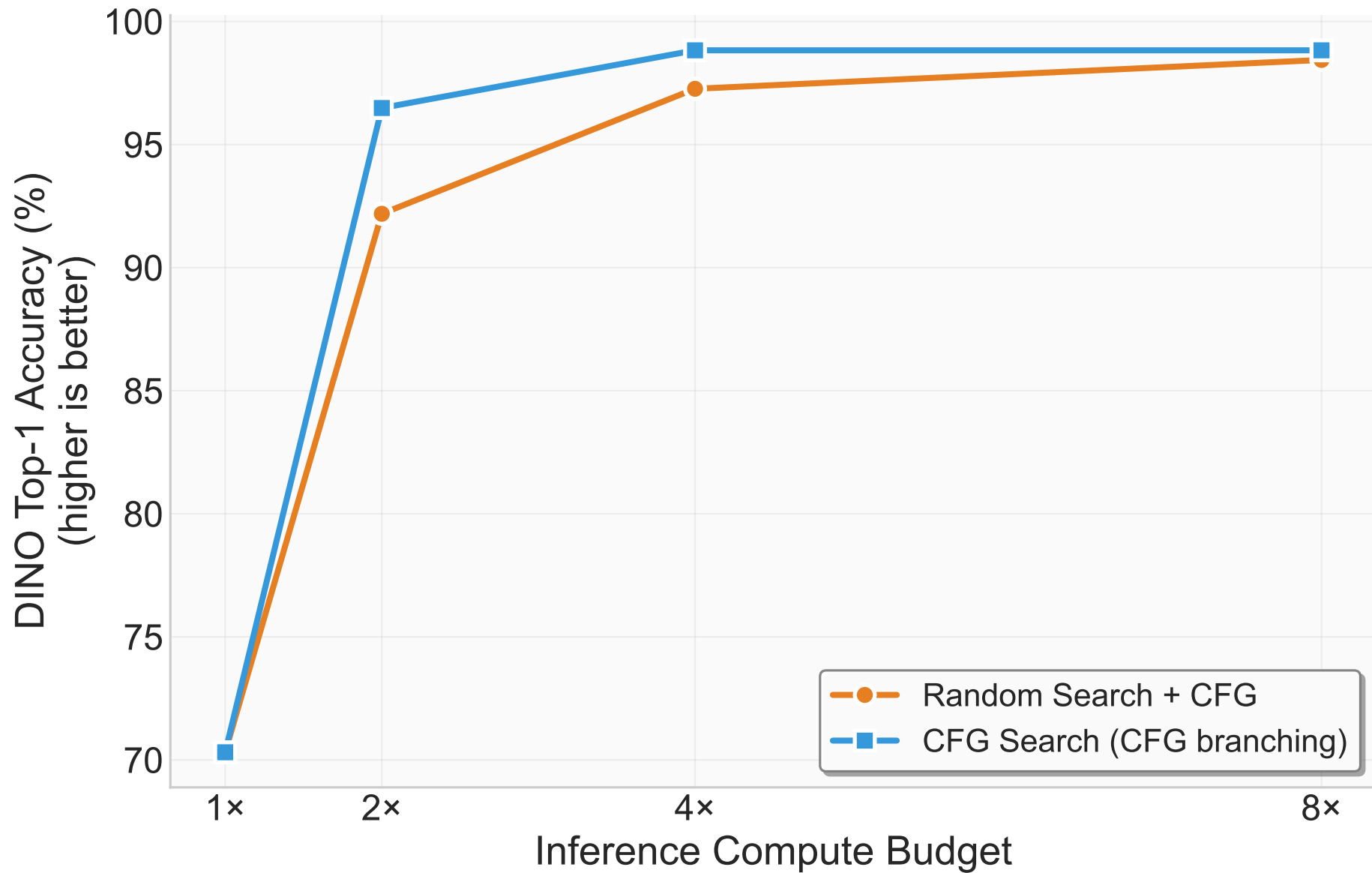
CFG Search Ablation: DINO Top-1 Accuracy (%)
