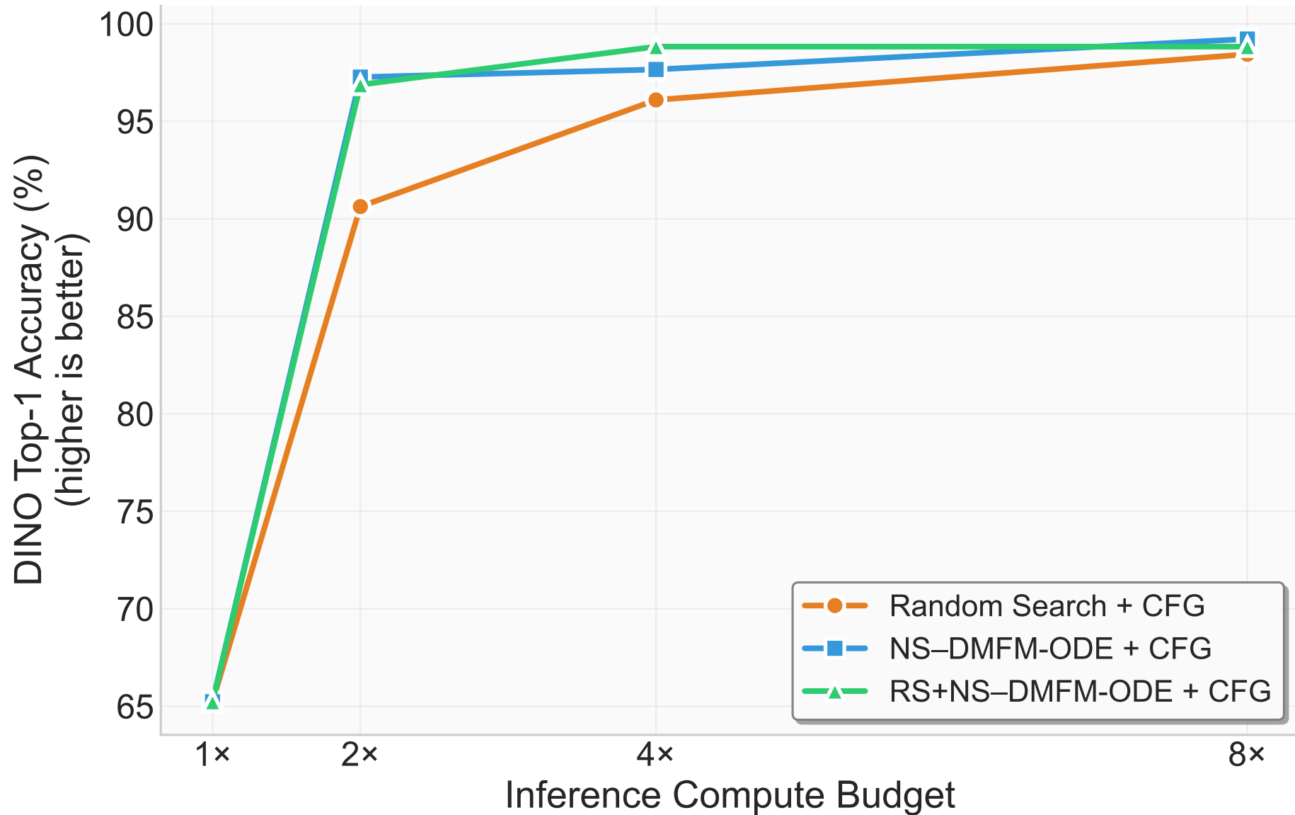
CFG Ablation (scale=1.5): DINO Top-1 Accuracy (%)
