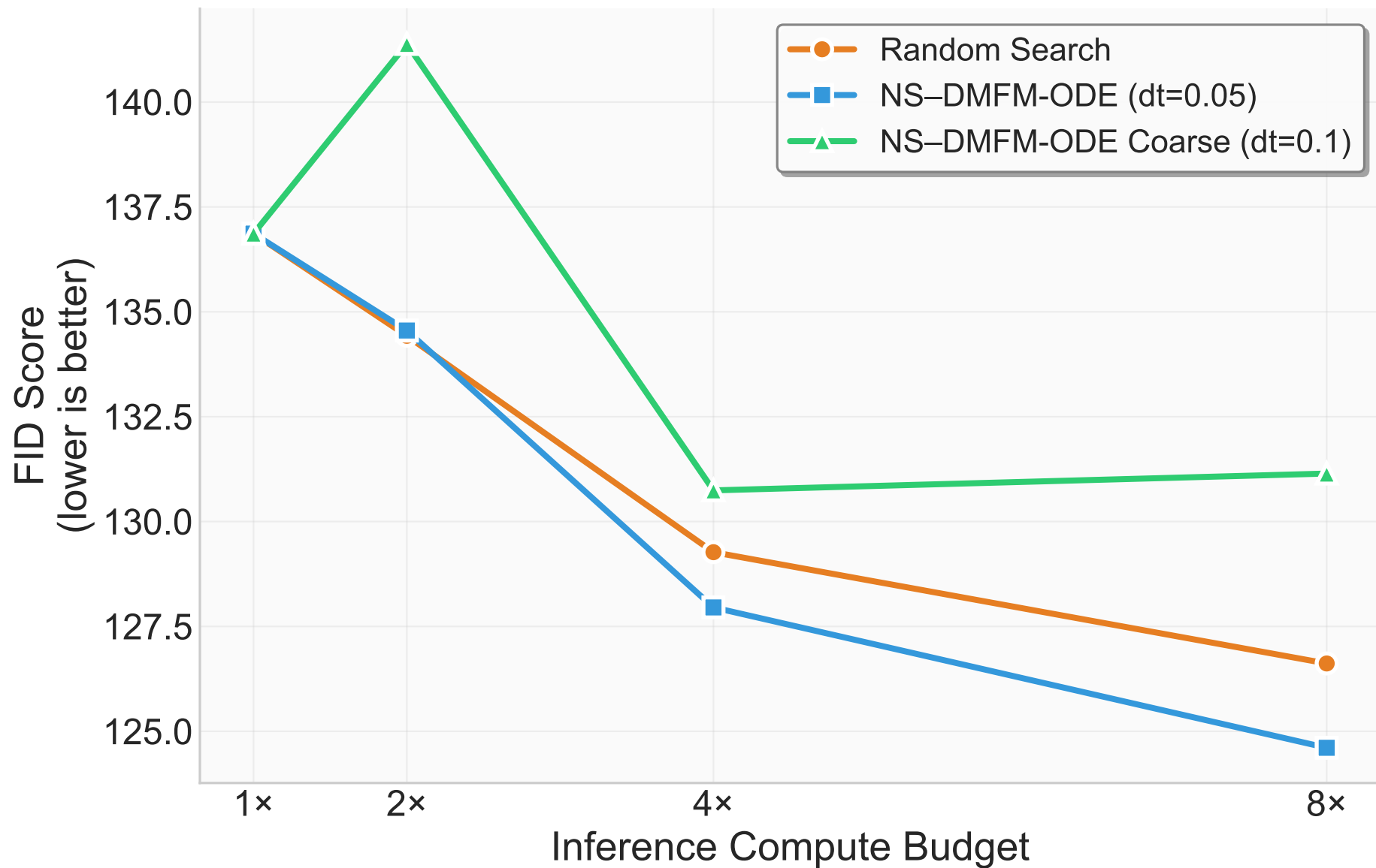
Coarse Simulate Forward Ablation: FID Score
