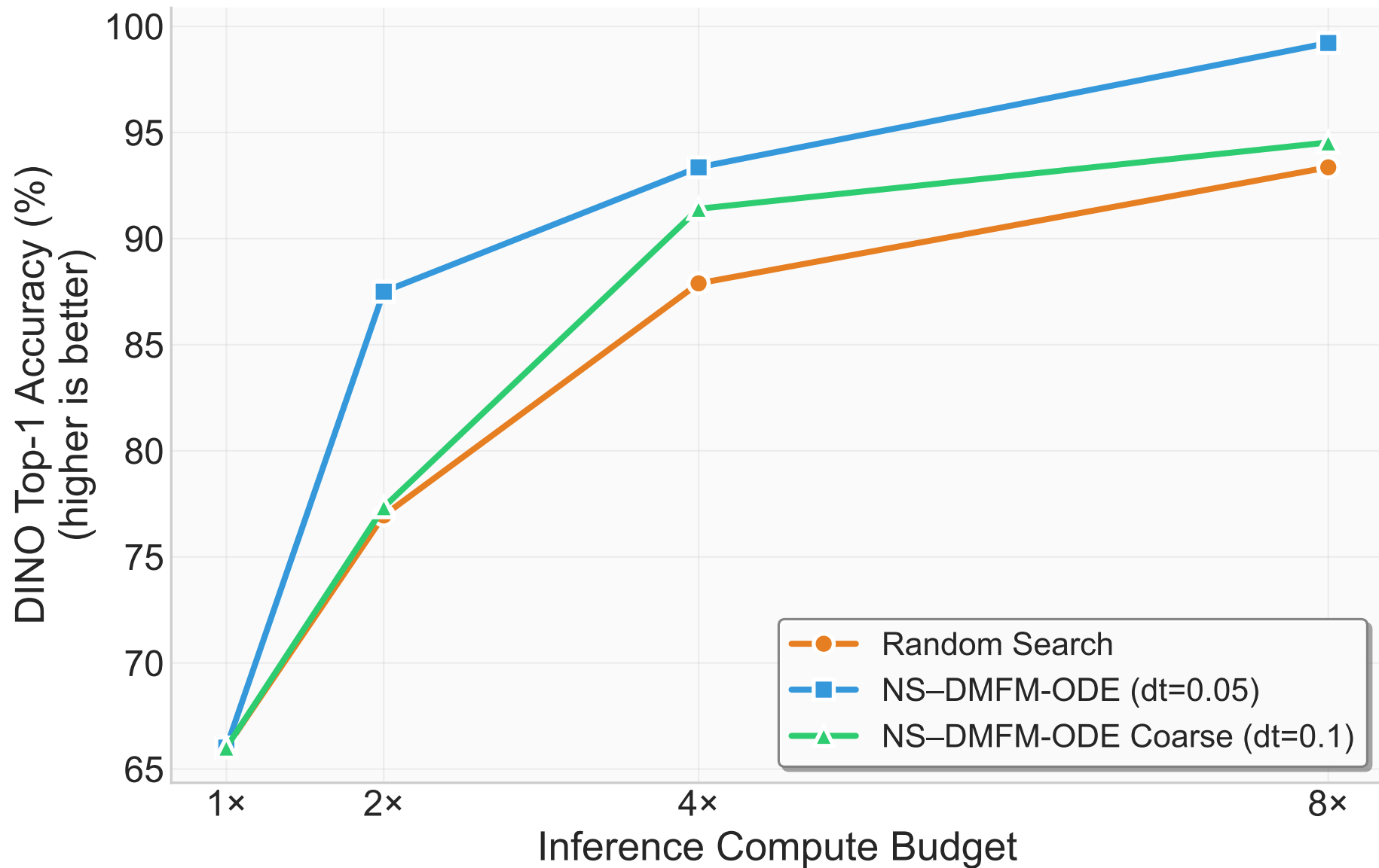
Coarse Simulate Forward Ablation: DINO Top-1 Accuracy (%)
