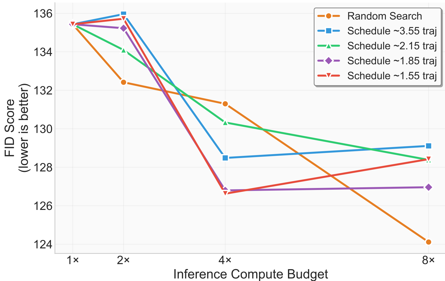
Branching Schedule Ablation: FID Score
