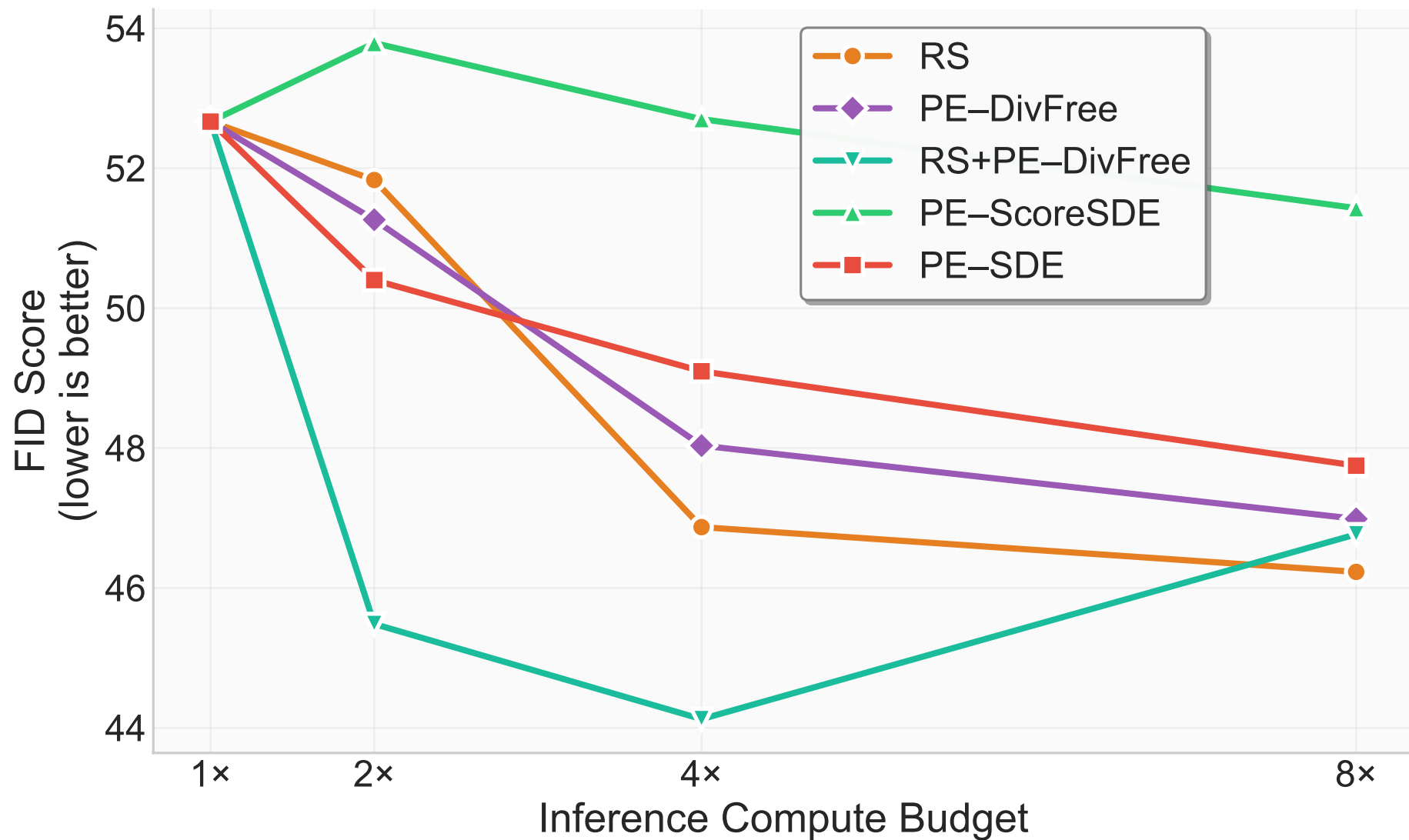
FID Score vs. Compute Budget DINO Verifier
