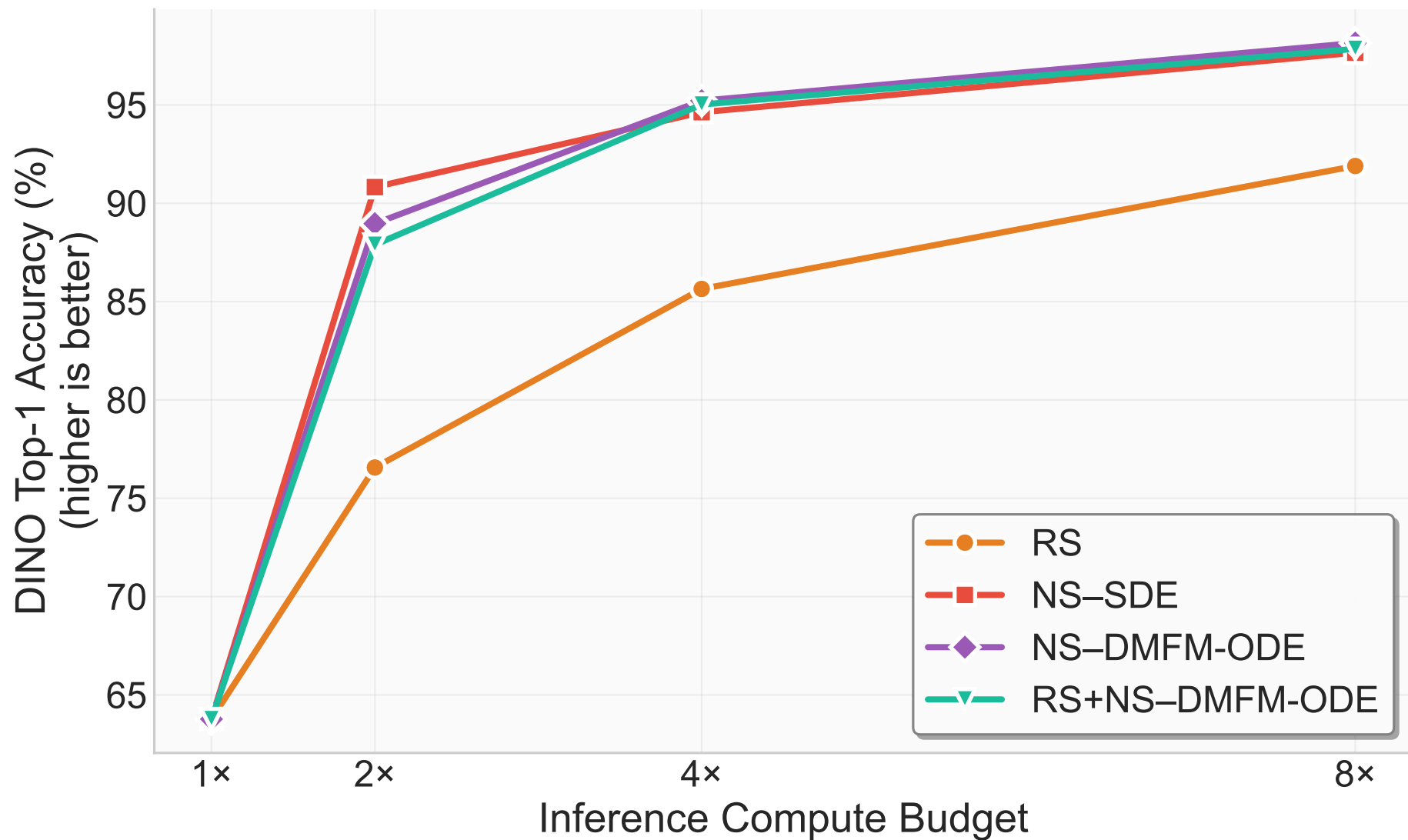
DINO Top-1 Accuracy (%) vs. Compute Budget DINO Verifier
