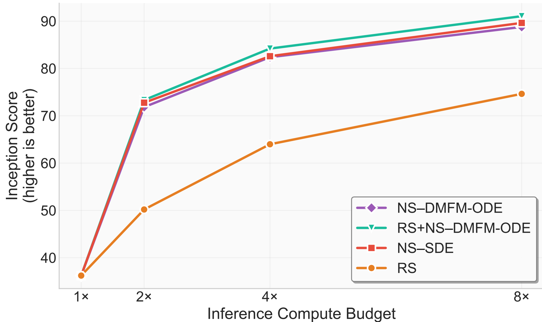
Inception Score vs. Compute Budget Inception Verifier
