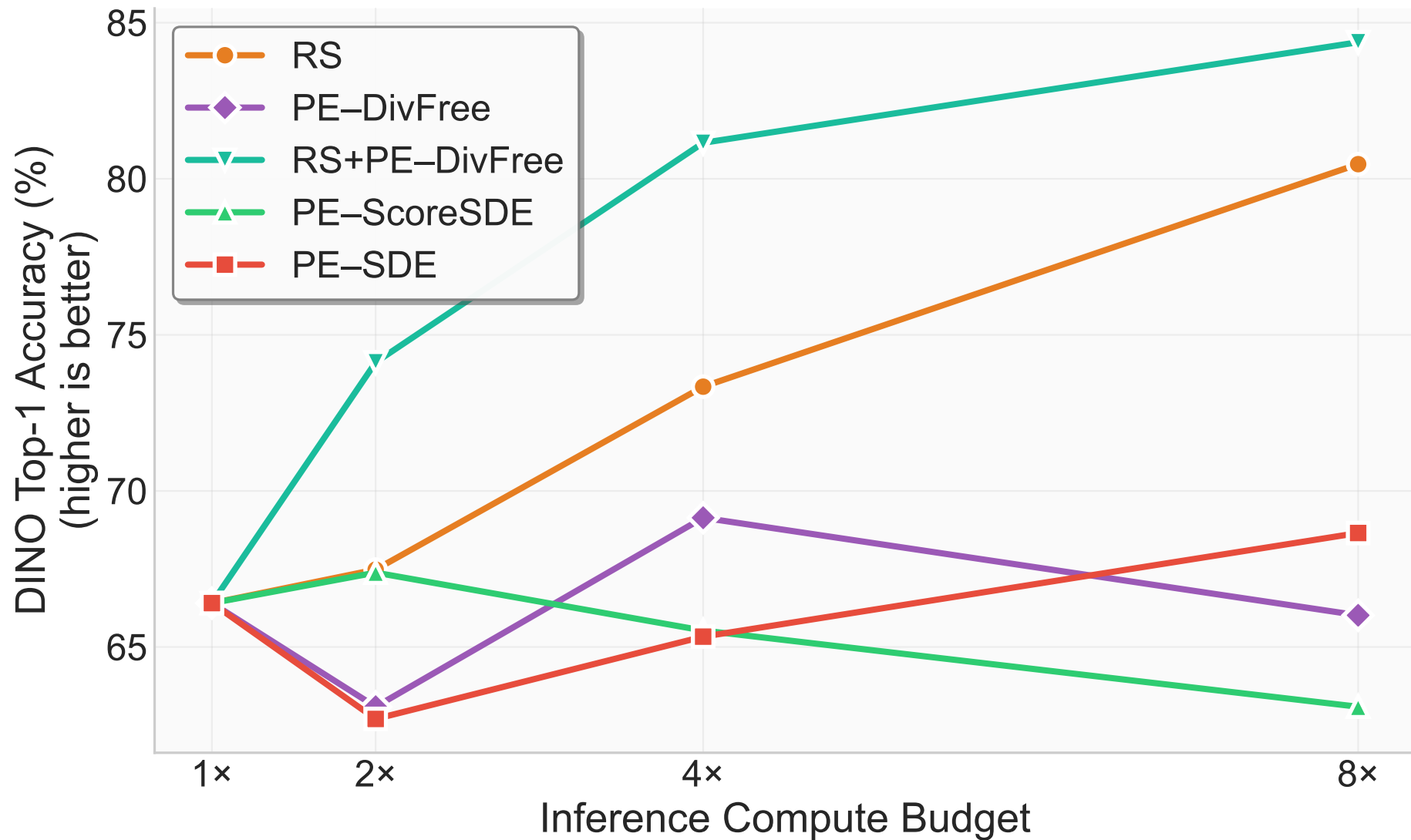
DINO Top-1 Accuracy (%) vs. Compute Budget Inception Verifier
