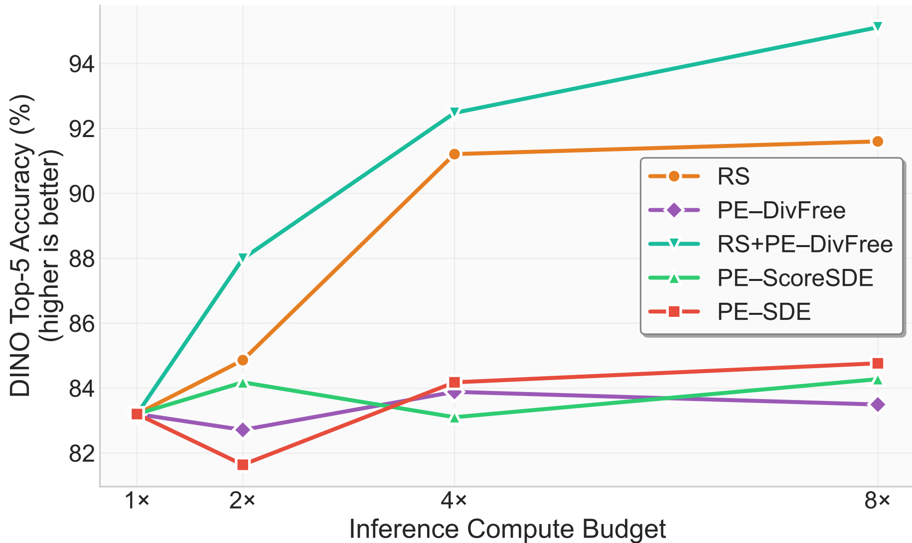
DINO Top-5 Accuracy (%) vs. Compute Budget Inception Verifier
