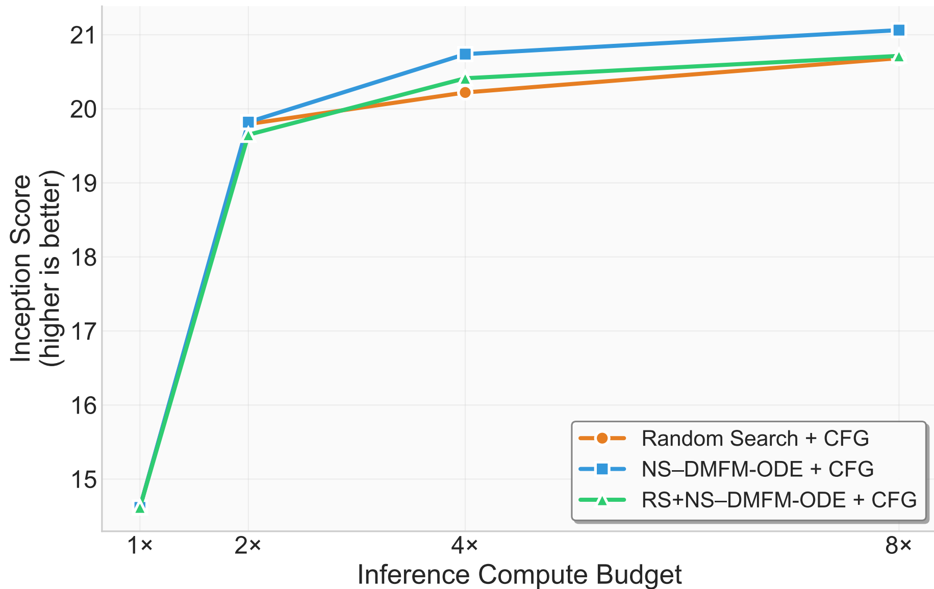
CFG Ablation (scale=1.5): Inception Score
