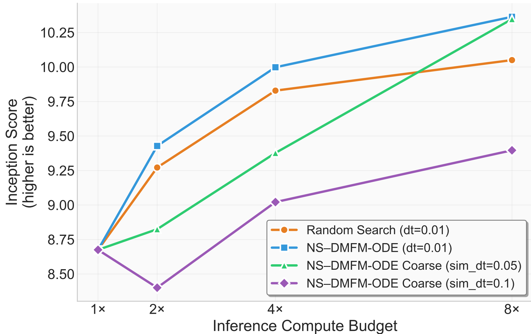
Coarse Simulate Forward (dt=0.01): Inception Score
